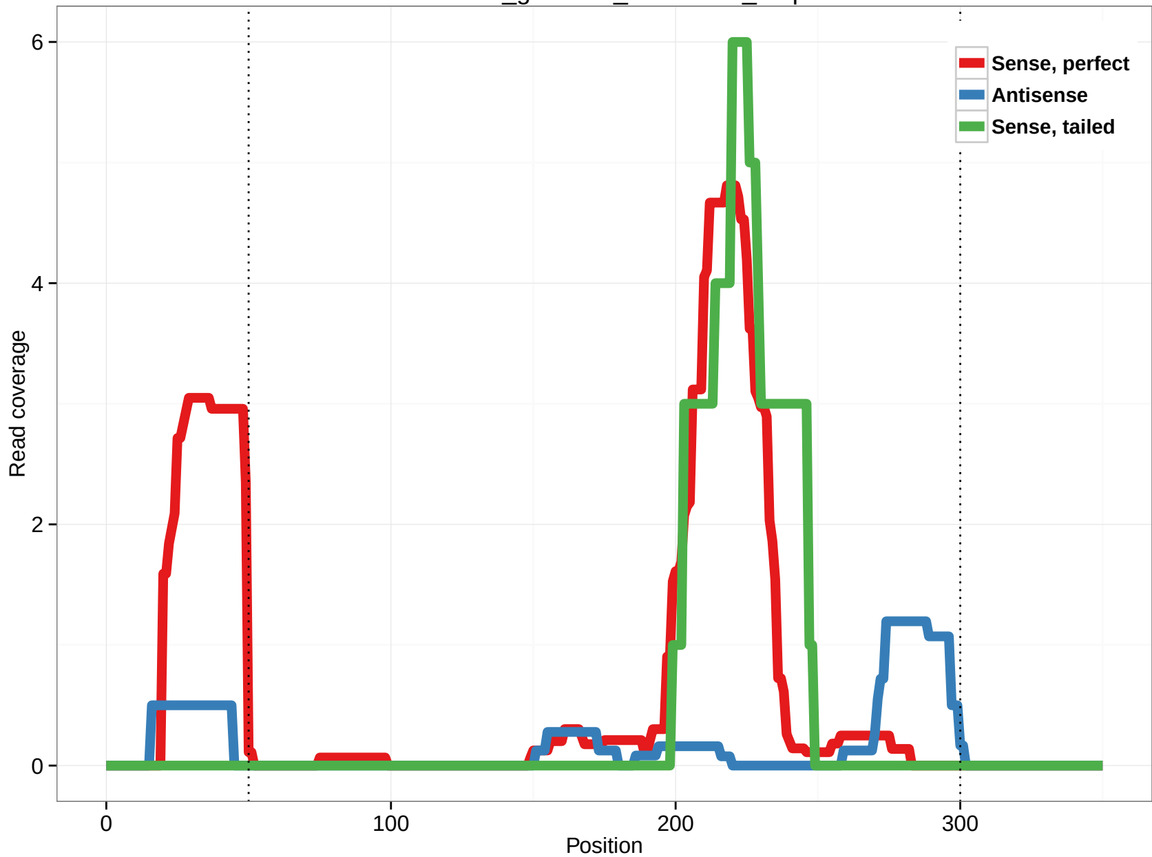
rheMac3_genscan_chr4.1548_7.3p
