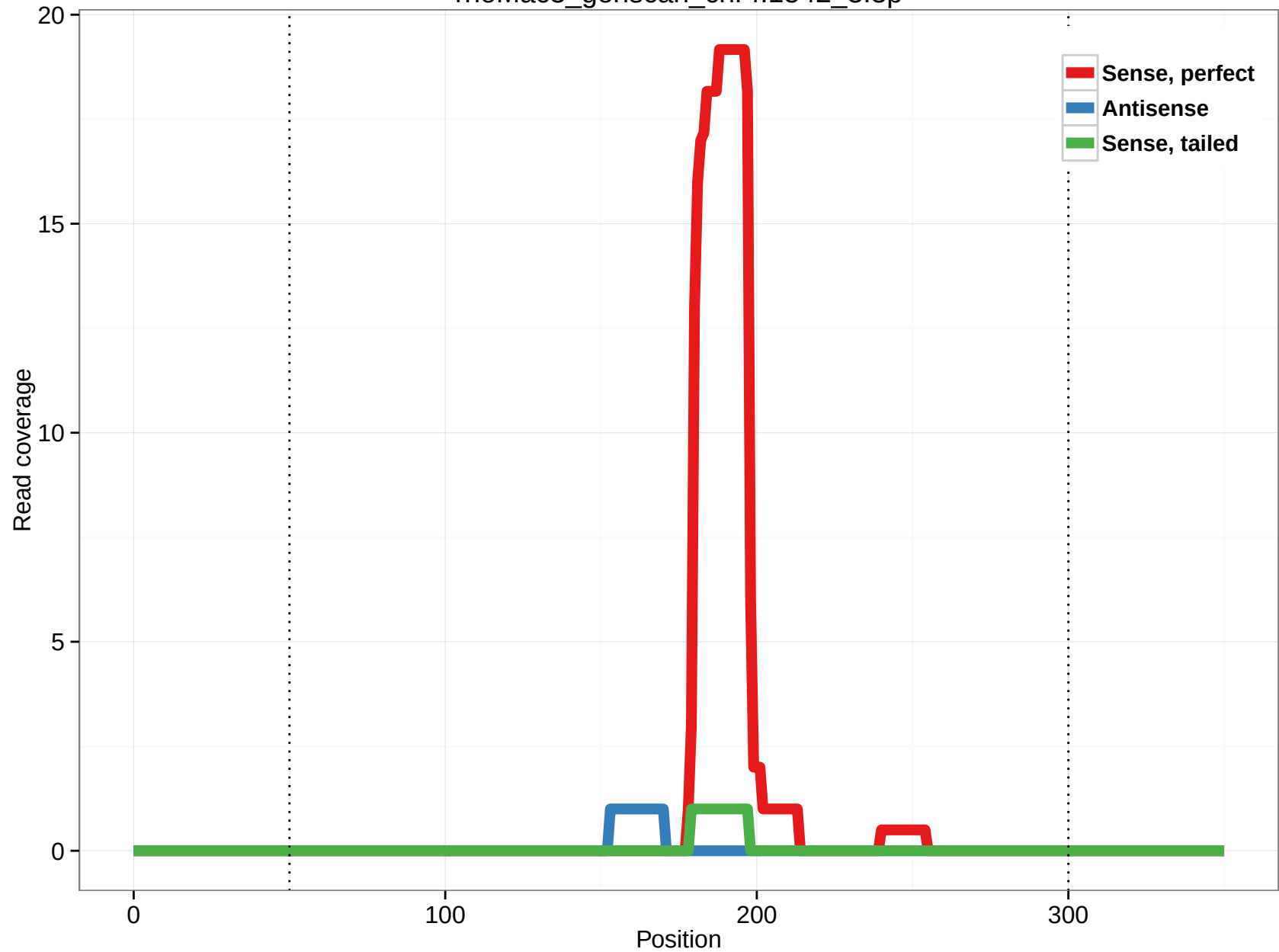
rheMac3_genscan_chr4.1542_3.3p
