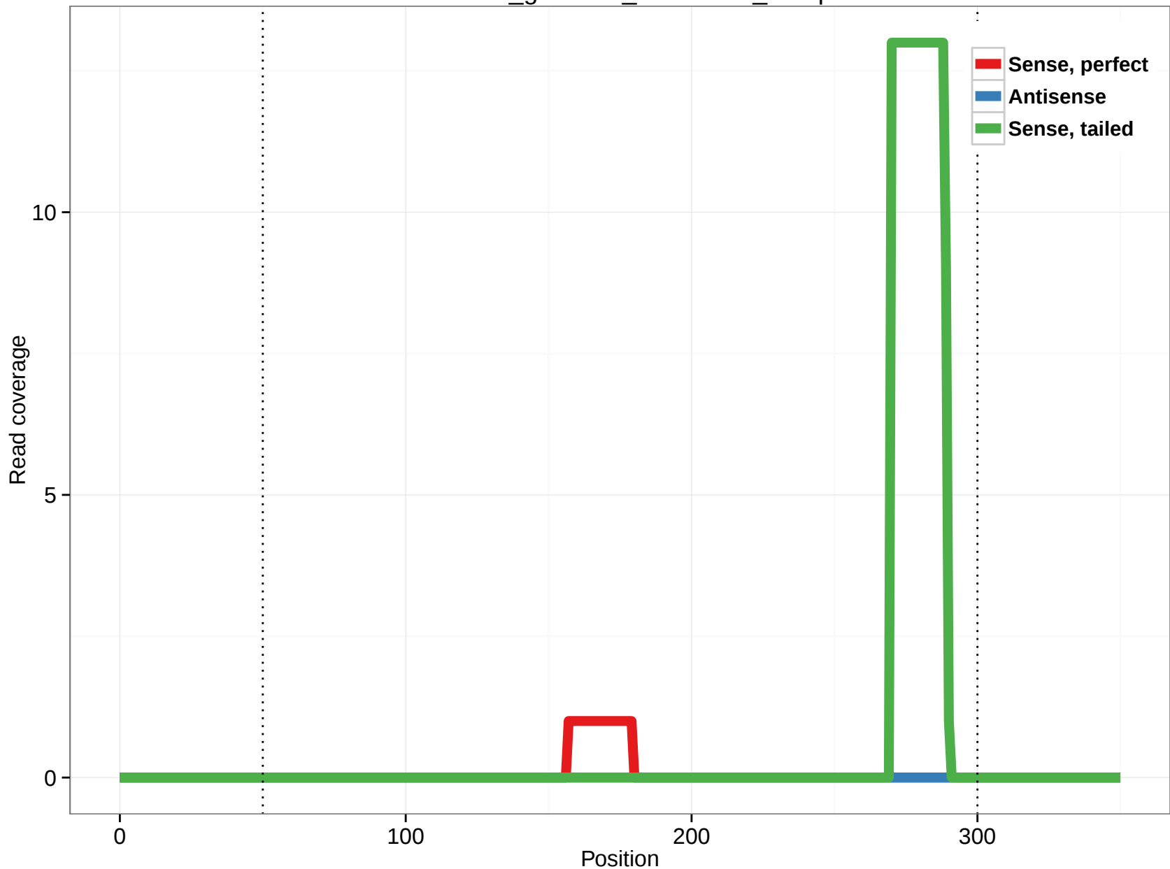
rheMac3_genscan_chr4.1495_13.3p
