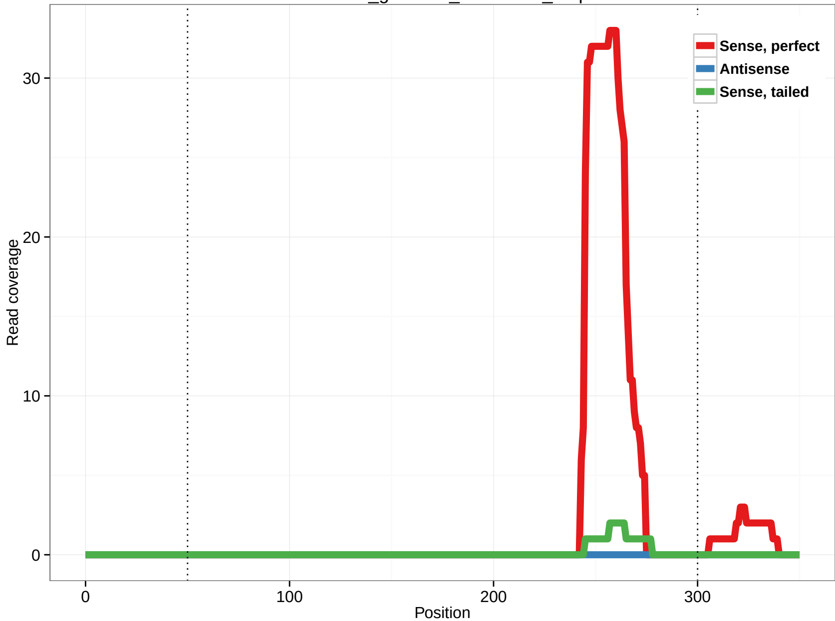
rheMac3_genscan_chr4.1429_5.3p
