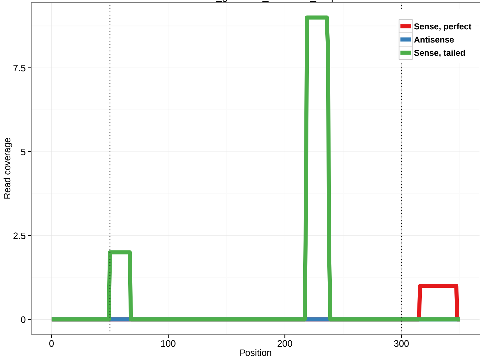
rheMac3_genscan_chr4.124_7.3p
