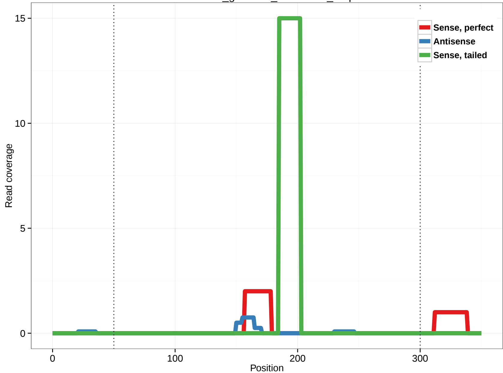
rheMac3_genscan_chr4.1241_0.3p
