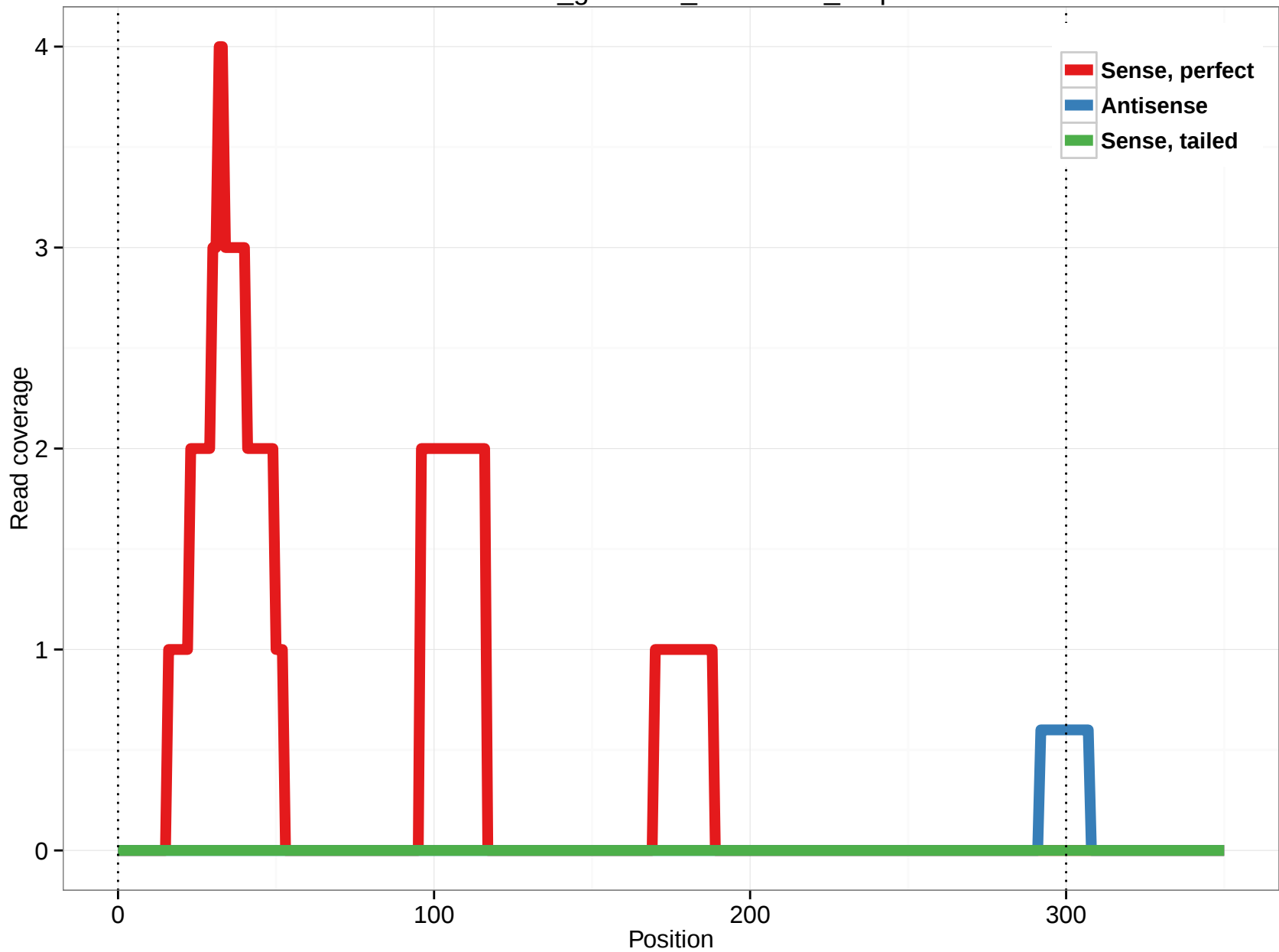
rheMac3_genscan_chr4.1220_1.3p
