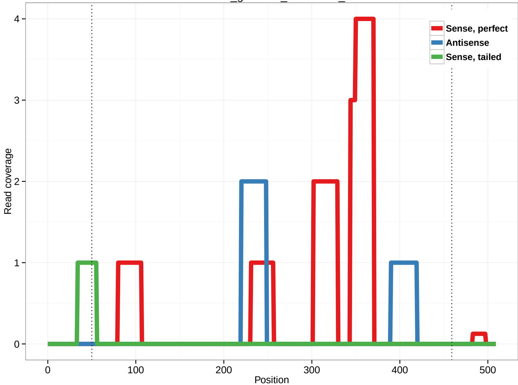
rheMac3_genscan_chr4.1090_17
