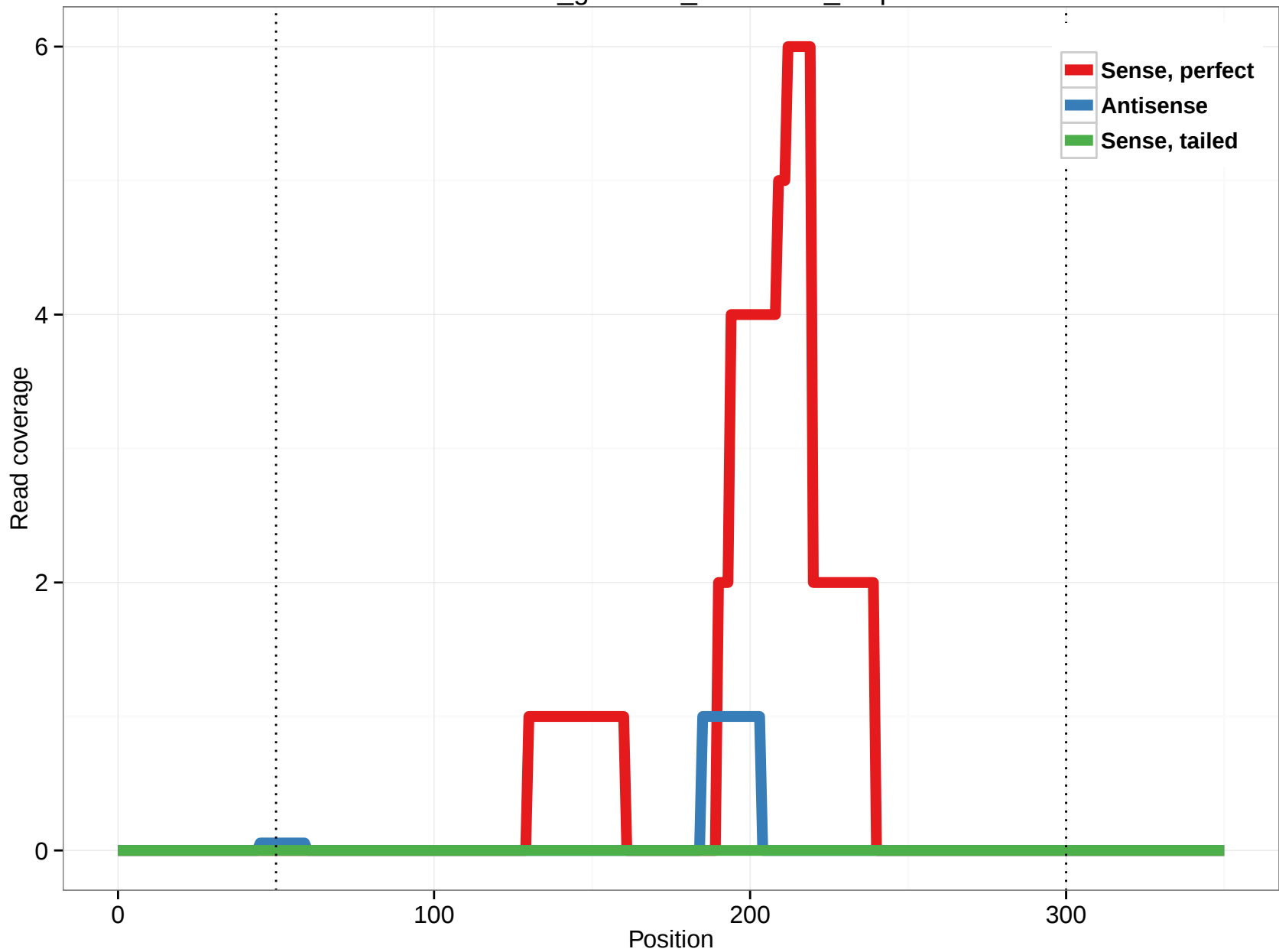
rheMac3_genscan_chr4.1087_4.3p
