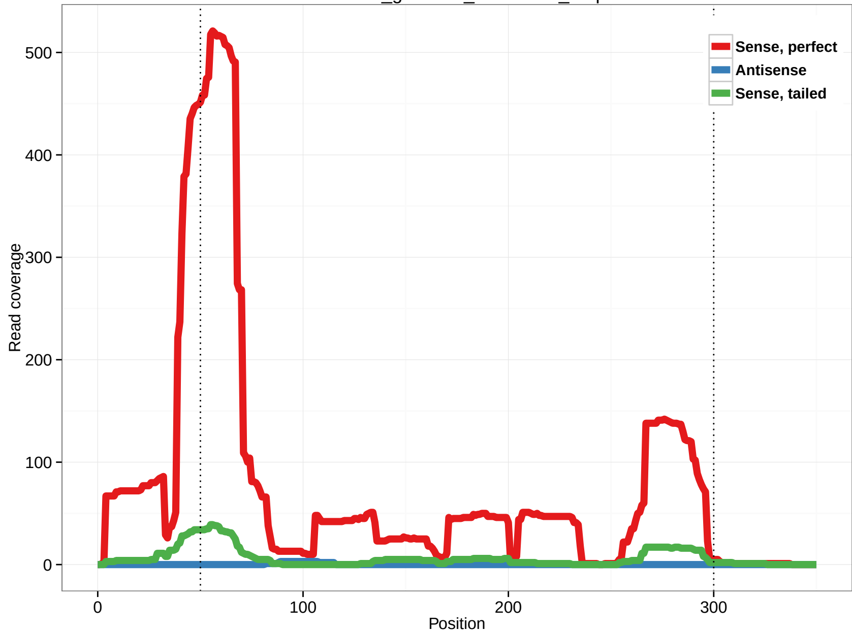
rheMac3_genscan_chr4.1087_0.5p
