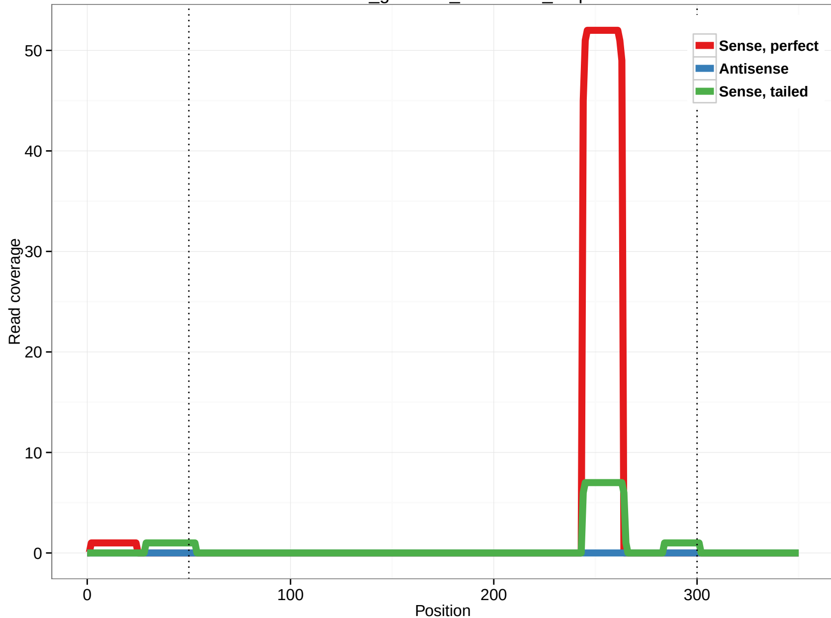
rheMac3_genscan_chr4.1048_1.5p
