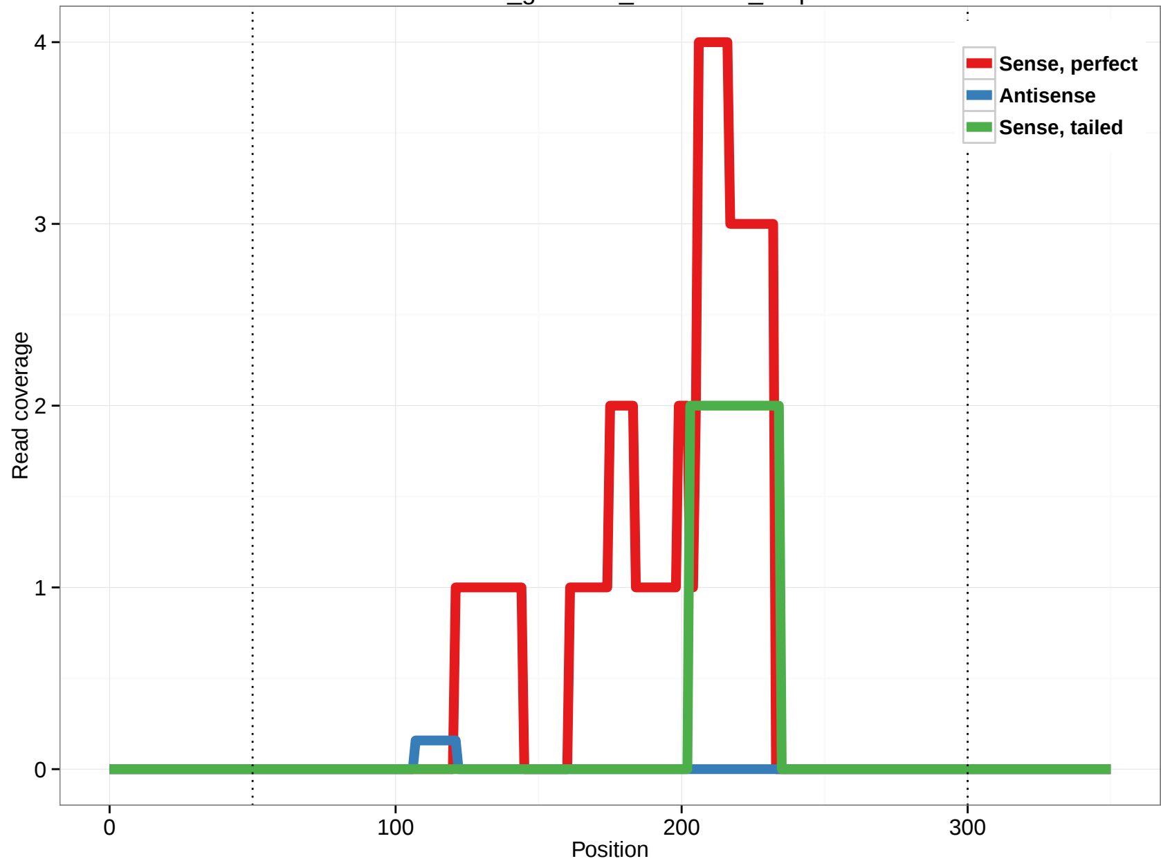
rheMac3_genscan_chr4.1022_8.5p
