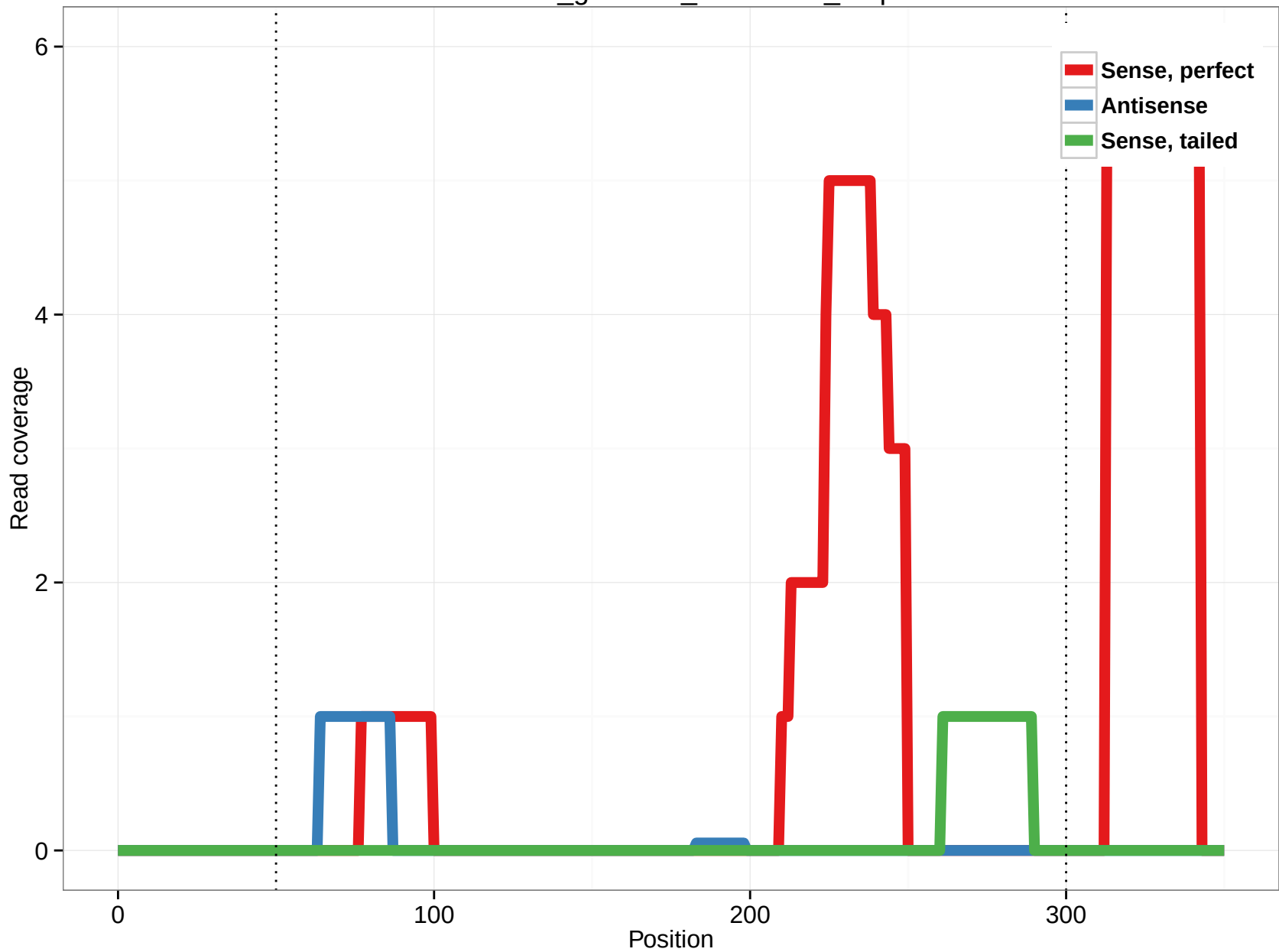
rheMac3_genscan_chr4.1020_0.5p
