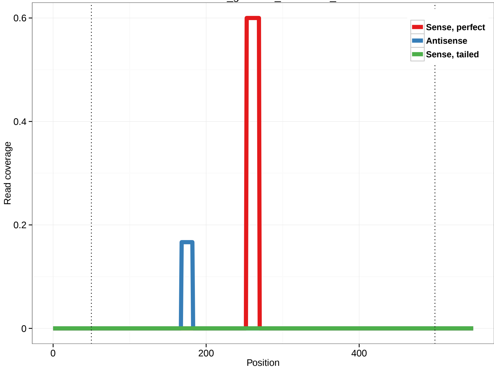
rheMac3_genscan_chr4.1017_1
