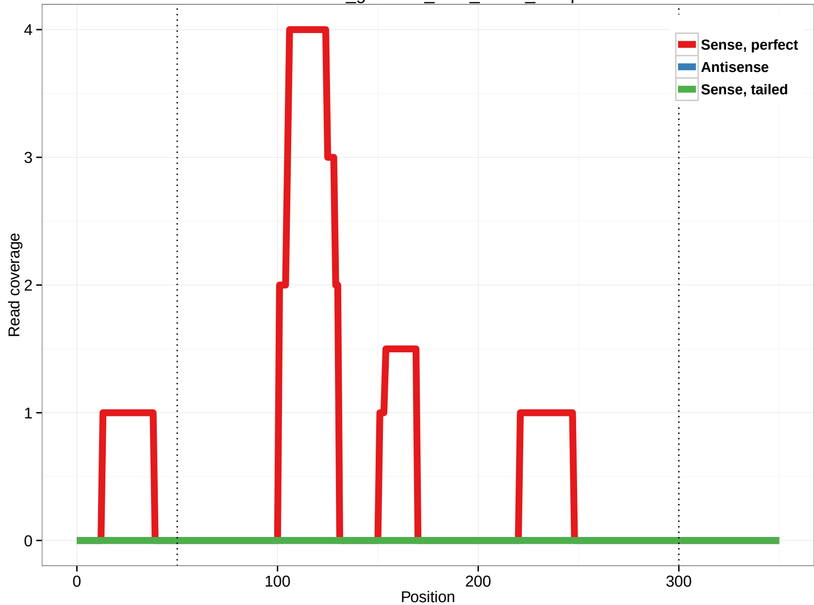
rheMac3_genscan_chr3_98.36_12.5p
