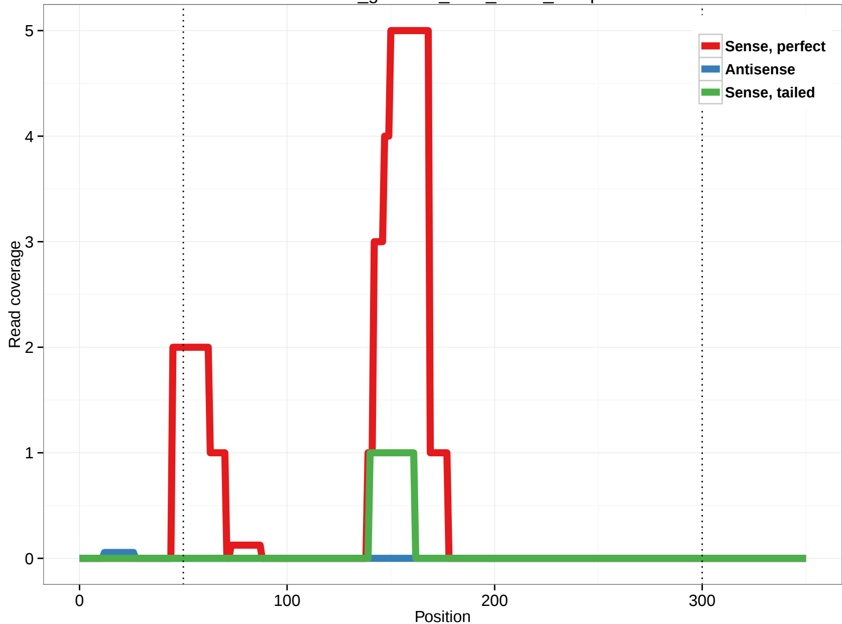
rheMac3_genscan_chr3_98.36_11.5p
