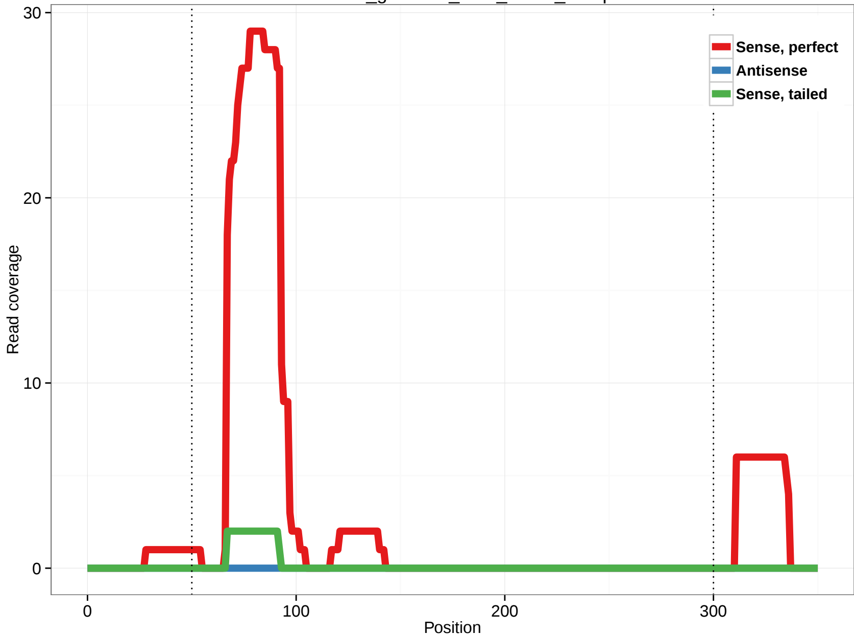
rheMac3_genscan_chr3_98.36_11.3p
