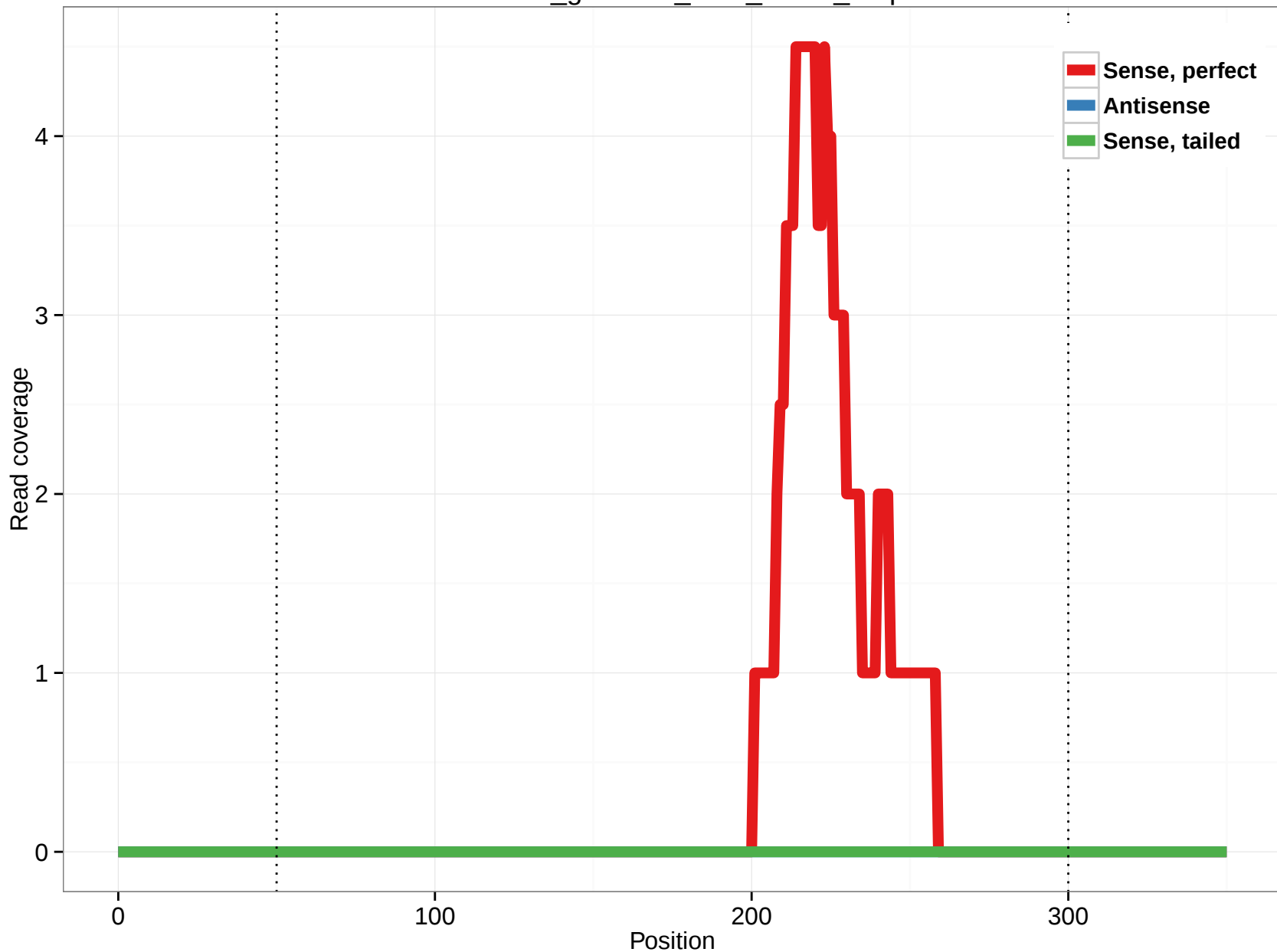
rheMac3_genscan_chr3_98.26_0.5p
