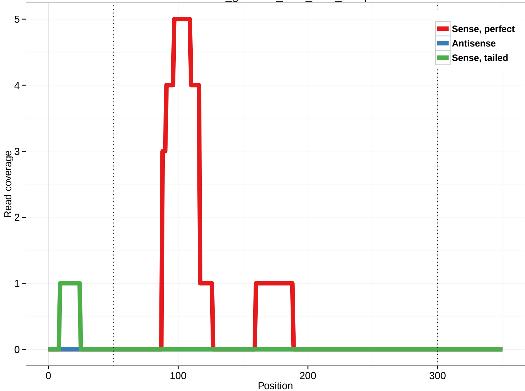
rheMac3_genscan_chr3_98.1_22.5p
