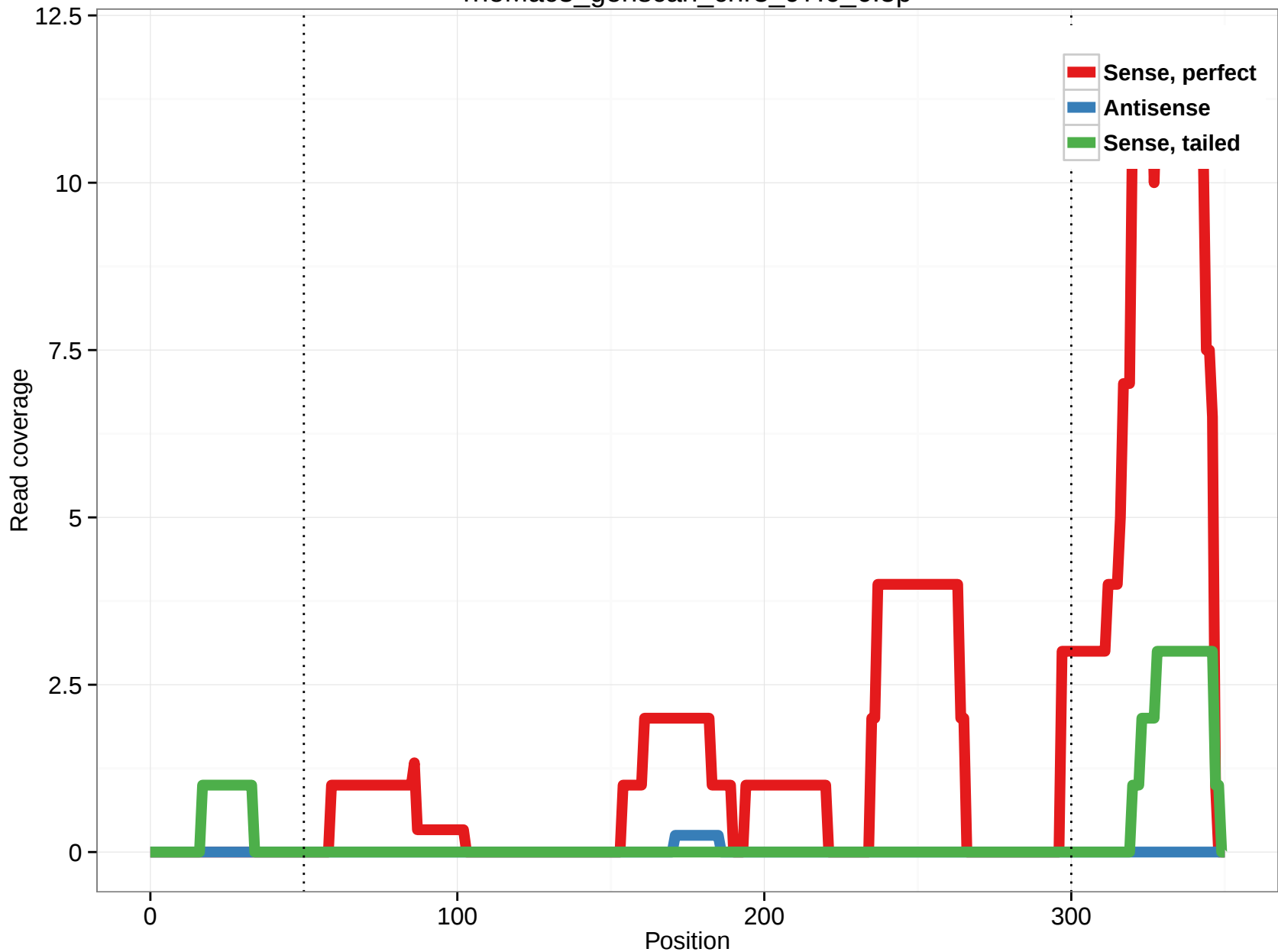
rheMac3_genscan_chr3_97.6_6.5p
