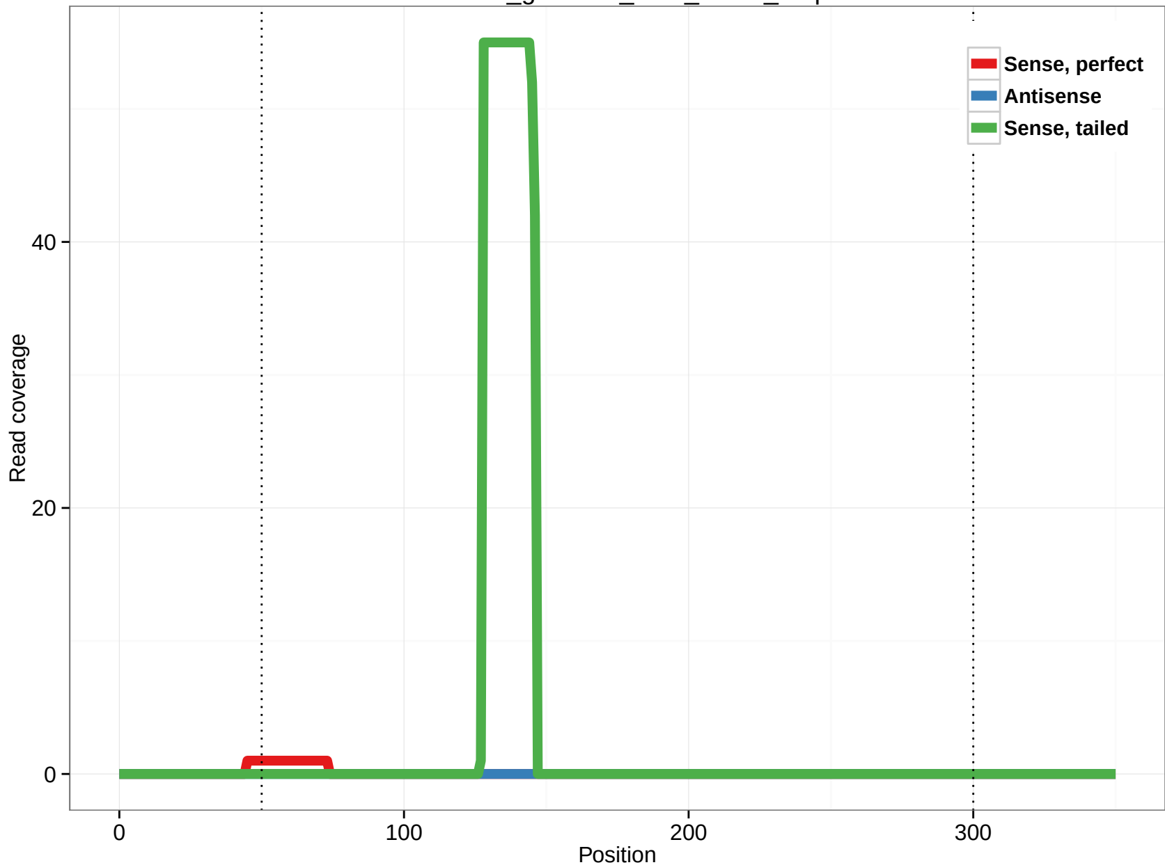
rheMac3_genscan_chr3_96.16_6.5p
