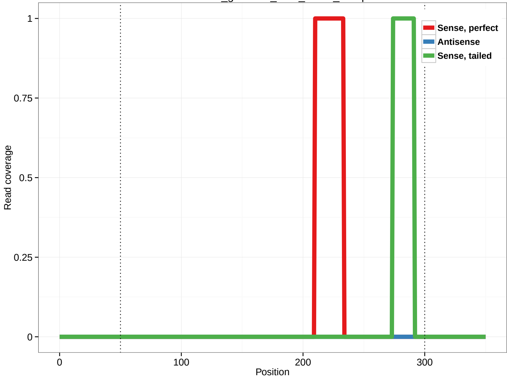
rheMac3_genscan_chr3_96.11_19.5p
