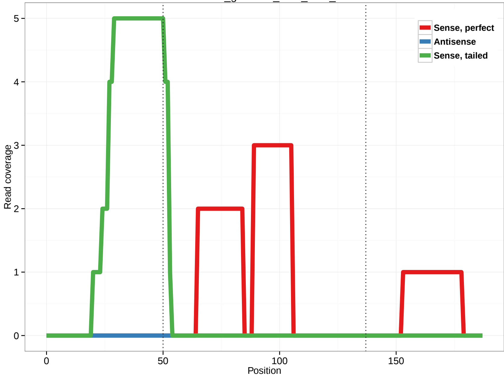
rheMac3_genscan_chr3_94.5_11
