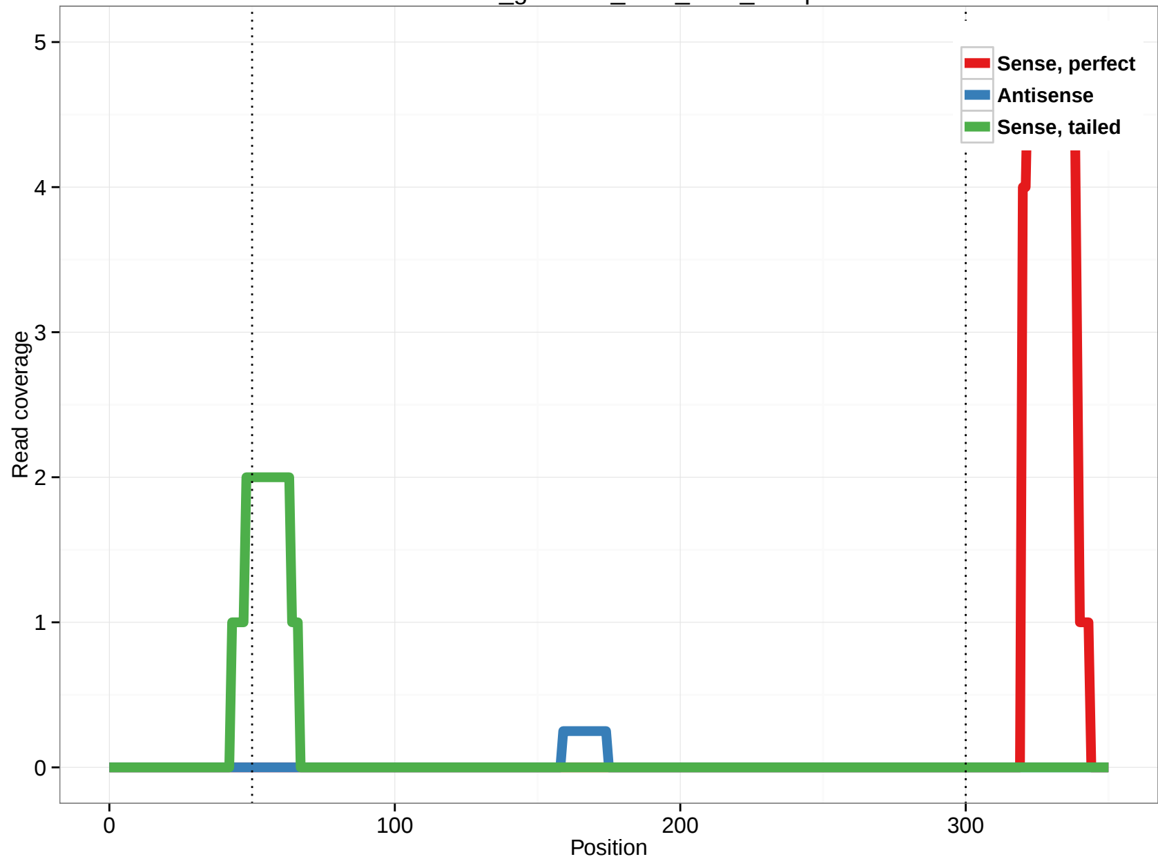
rheMac3_genscan_chr3_94.2_15.5p
