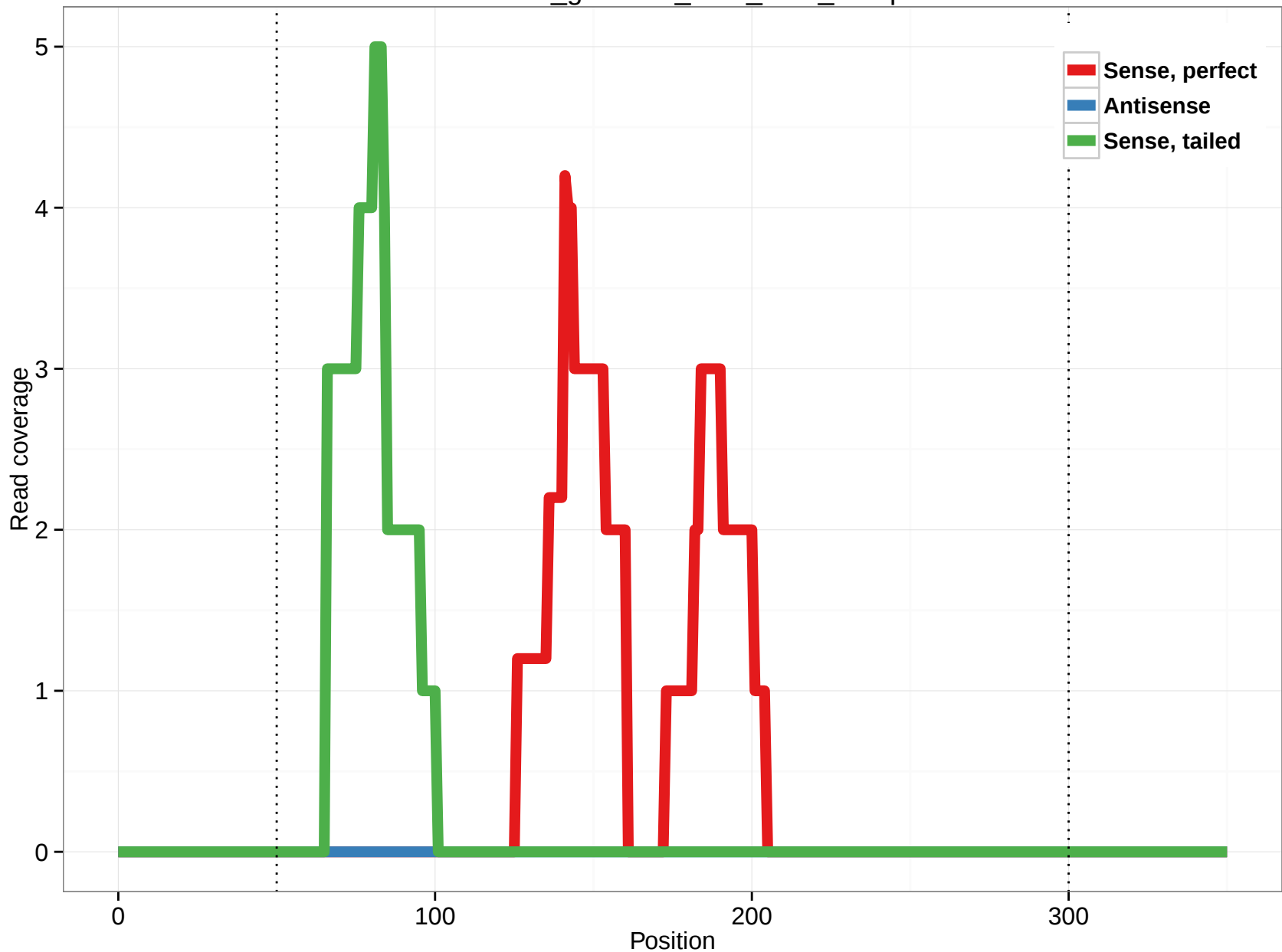
rheMac3_genscan_chr3_94.2_12.5p
