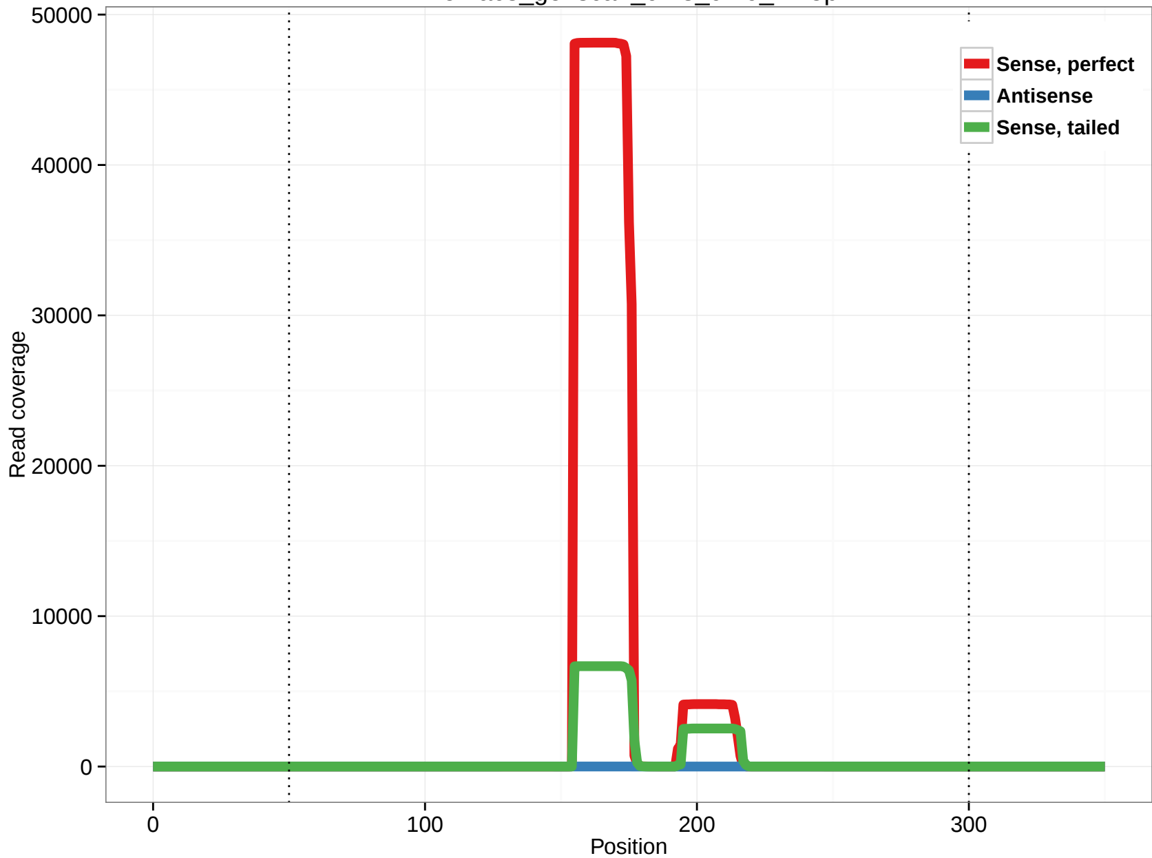
rheMac3_genscan_chr3_91.9_11.5p
