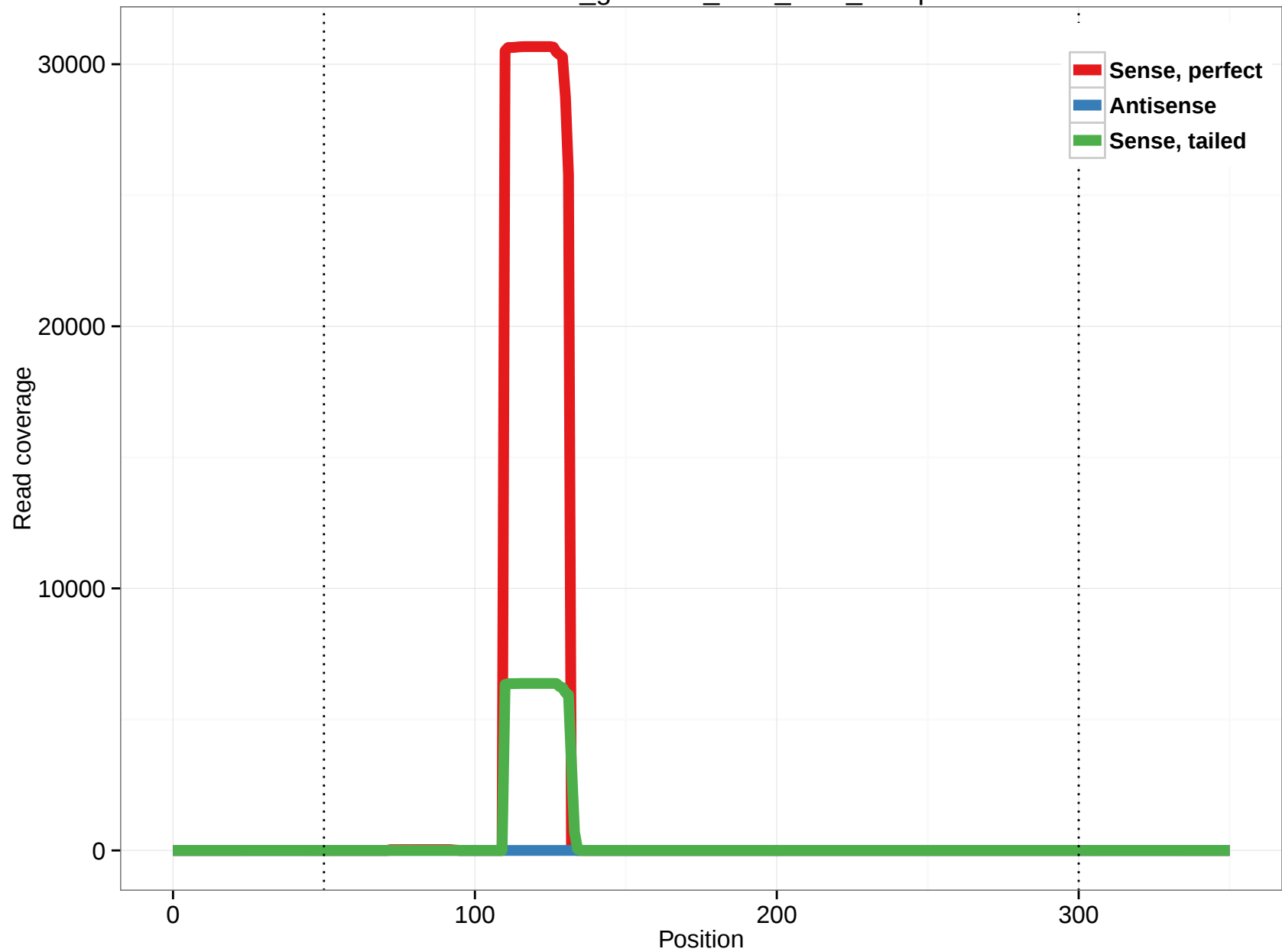
rheMac3_genscan_chr3_91.9_11.3p
