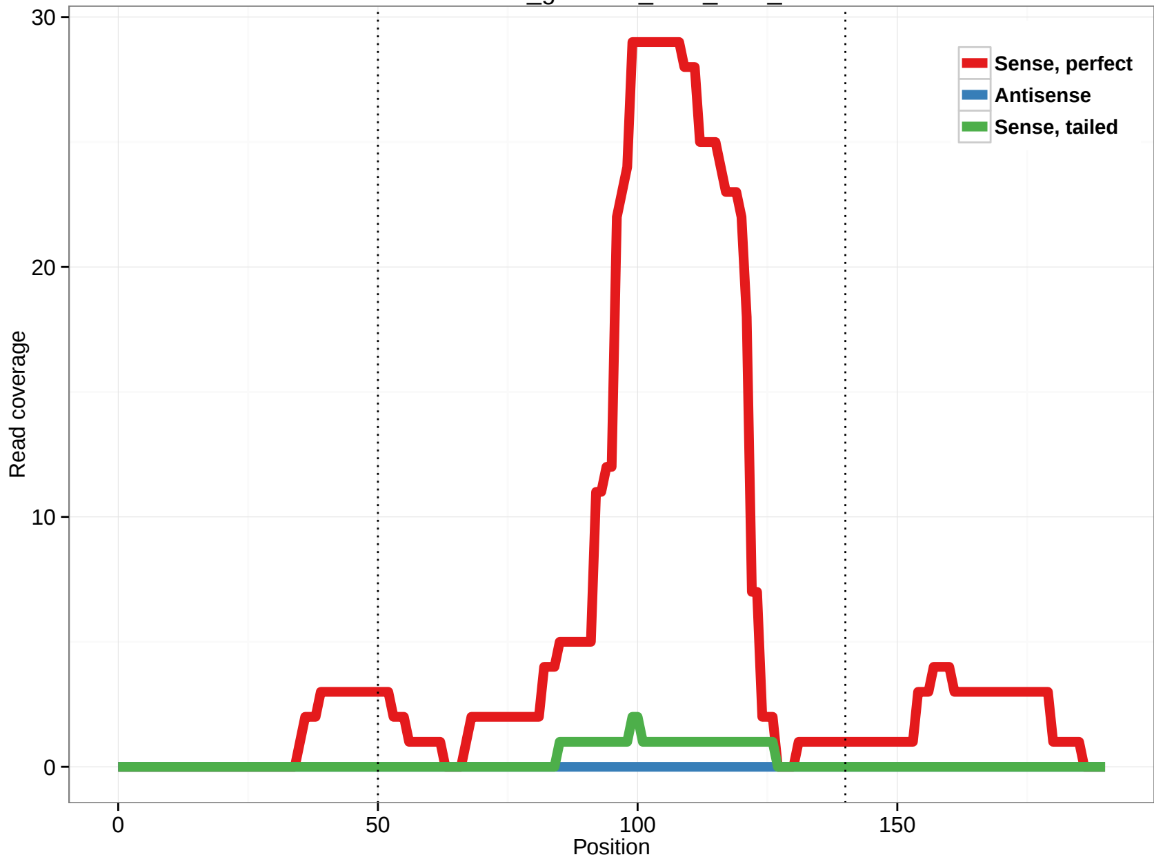
rheMac3_genscan_chr3_91.5_8
