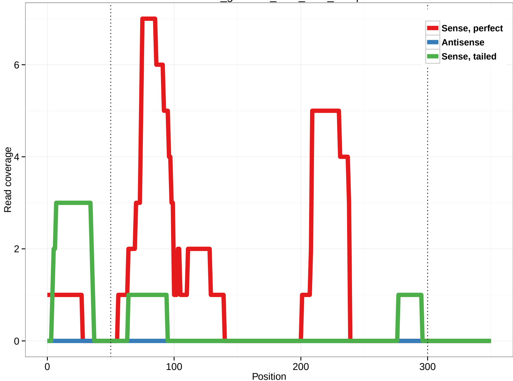
rheMac3_genscan_chr3_91.4_11.5p
