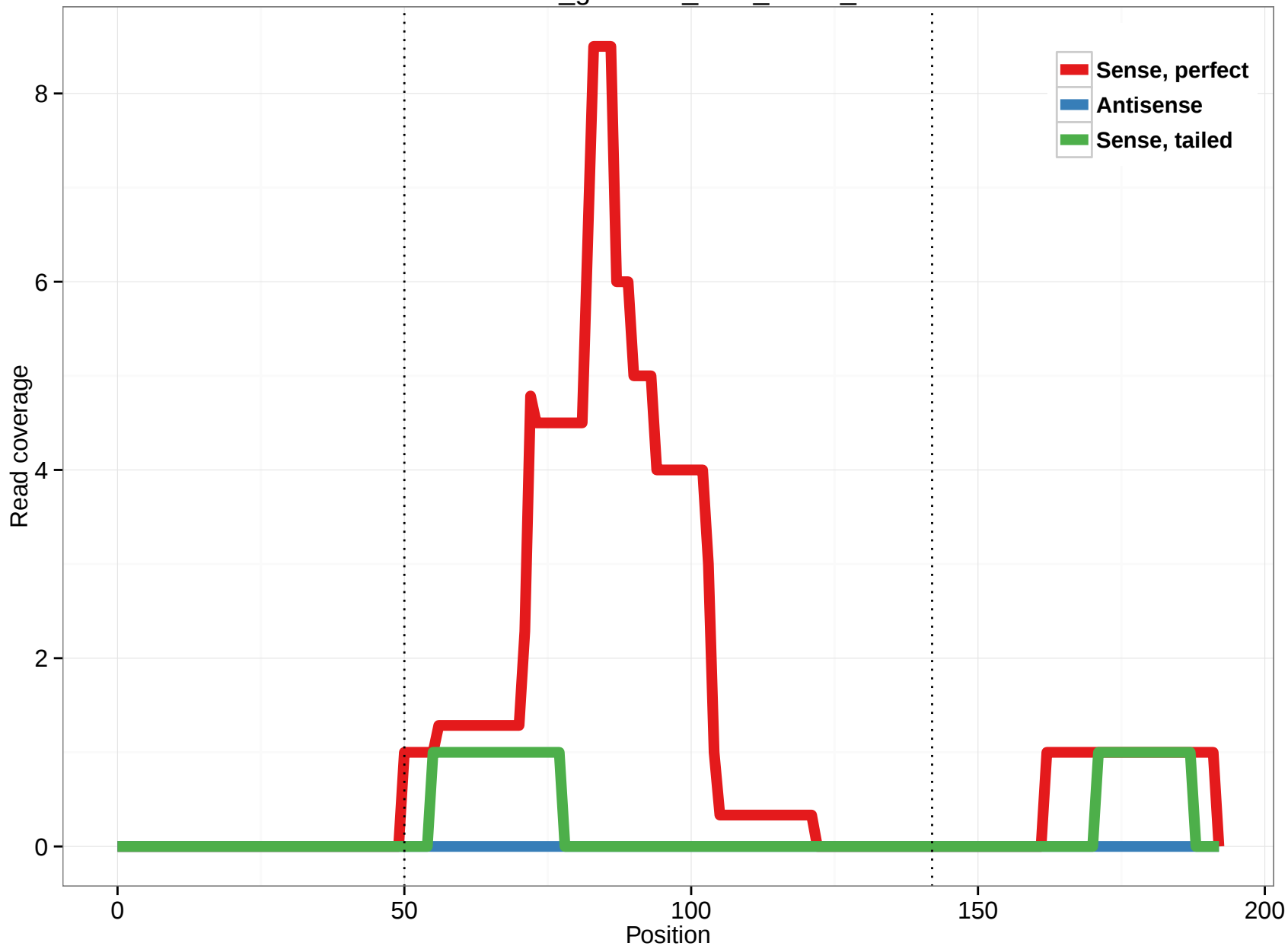
rheMac3_genscan_chr3_91.29_22
