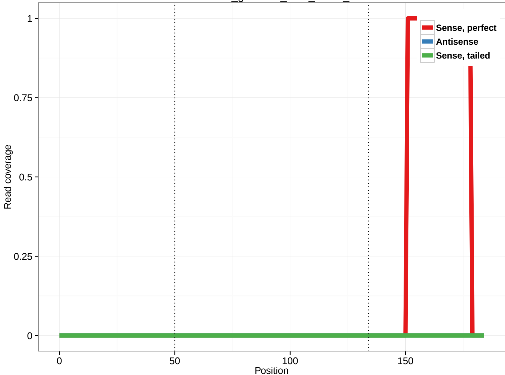
rheMac3_genscan_chr3_91.15_6
