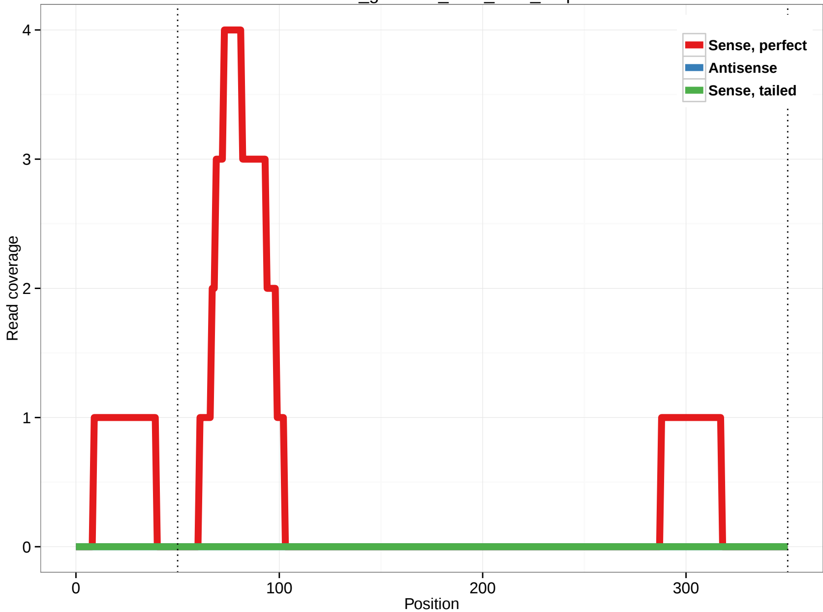
rheMac3_genscan_chr3_89.8_5.5p
