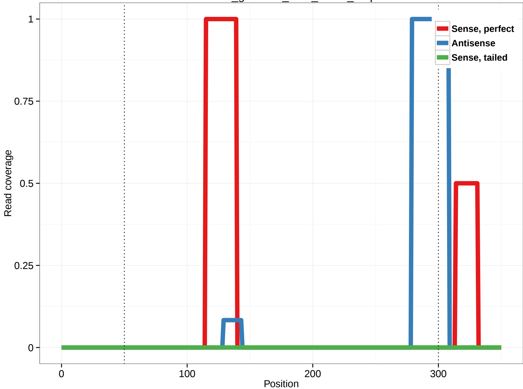
rheMac3_genscan_chr3_88.16_5.3p
