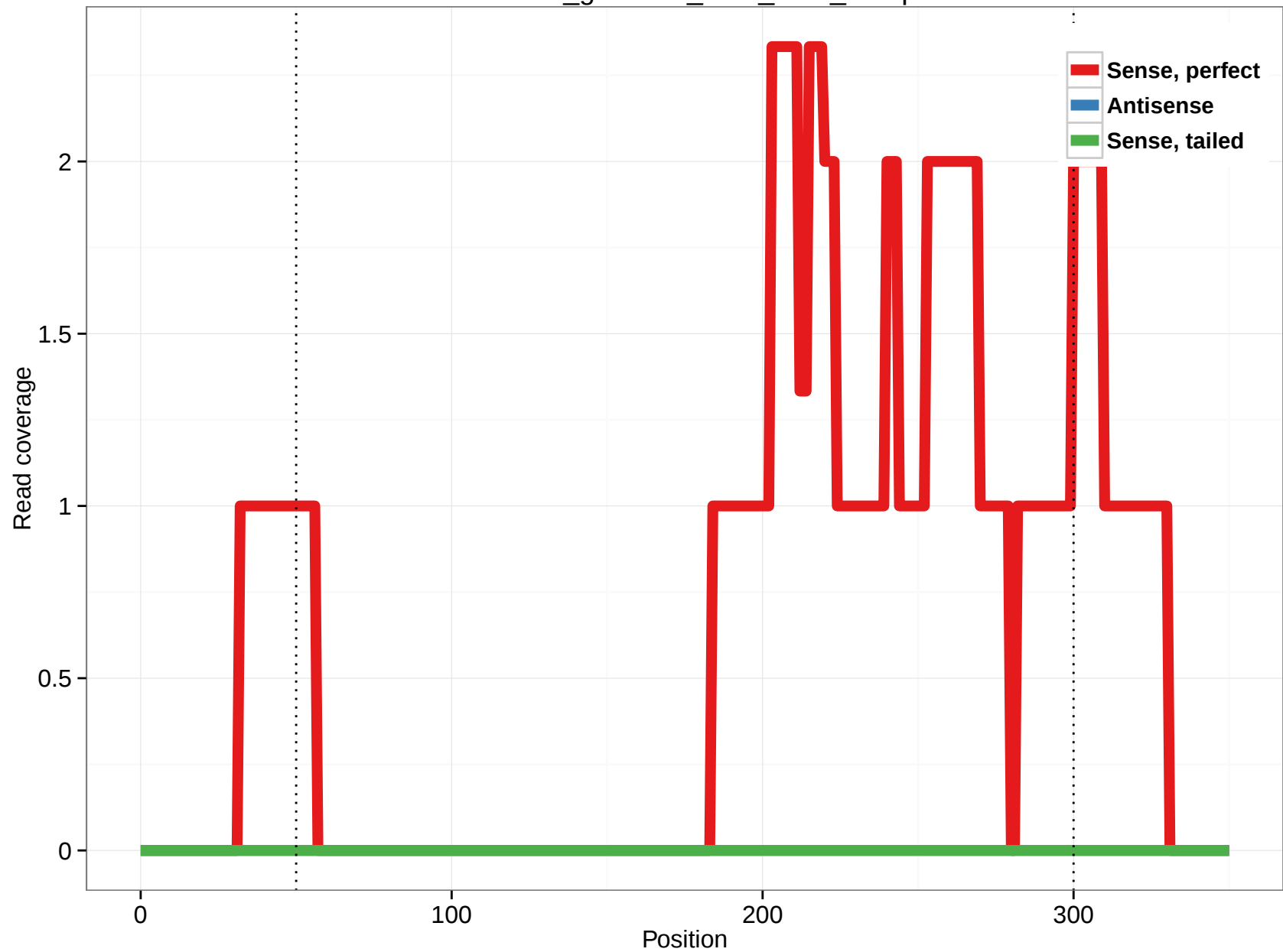
rheMac3_genscan_chr3_87.3_14.5p
