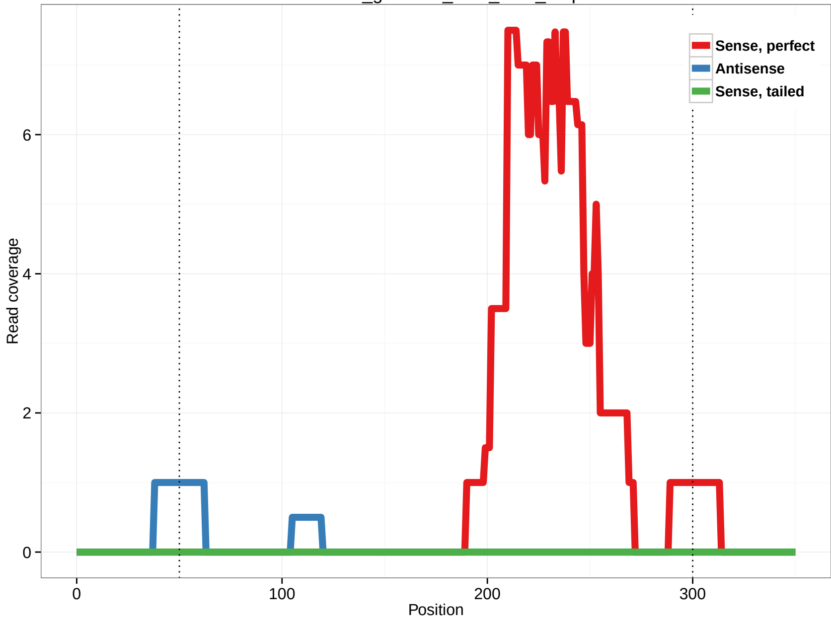
rheMac3_genscan_chr3_82.5_0.3p
