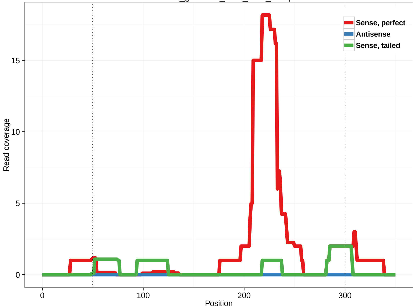
rheMac3_genscan_chr3_74.2_12.3p
