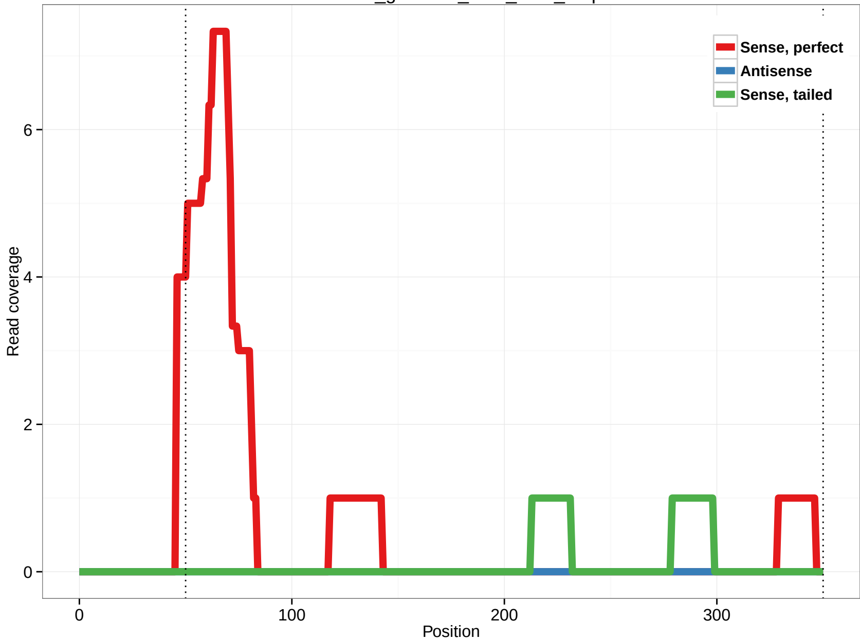
rheMac3_genscan_chr3_70.4_1.5p
