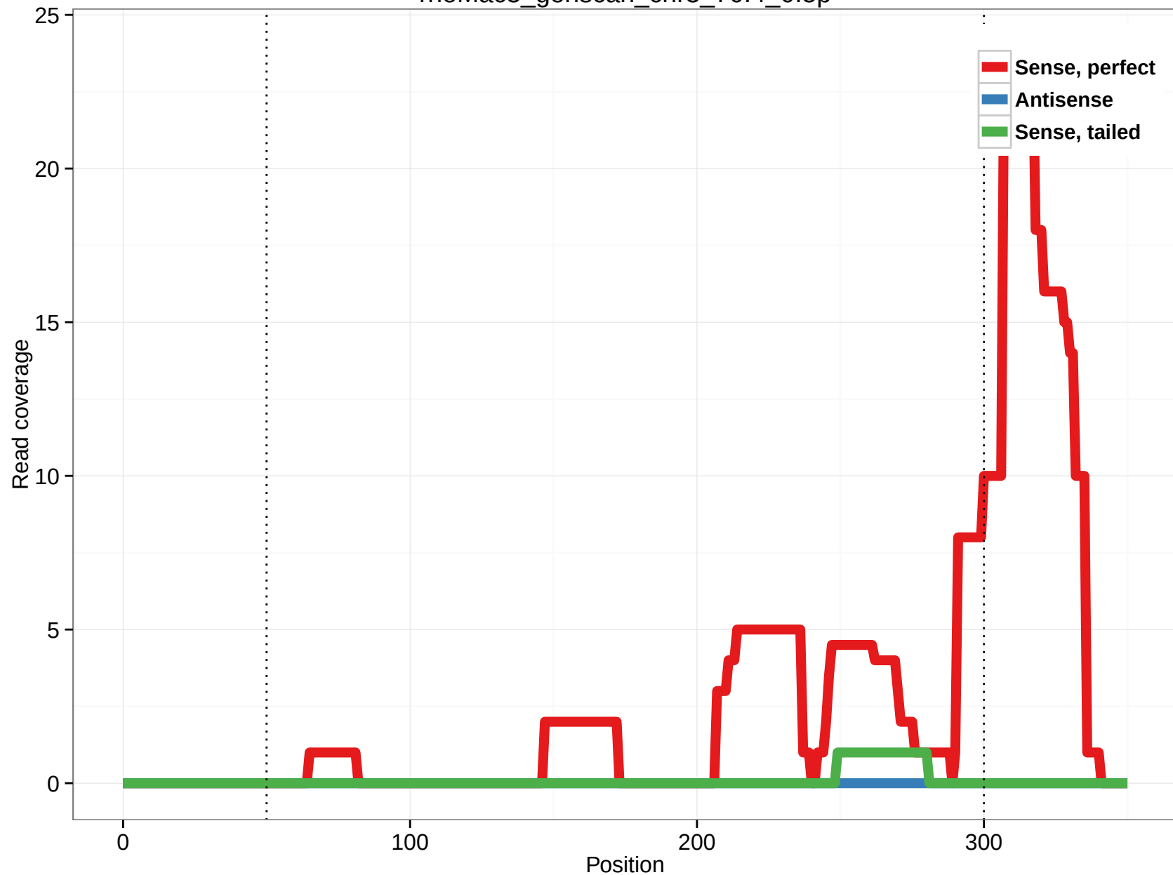
rheMac3_genscan_chr3_70.4_0.5p
