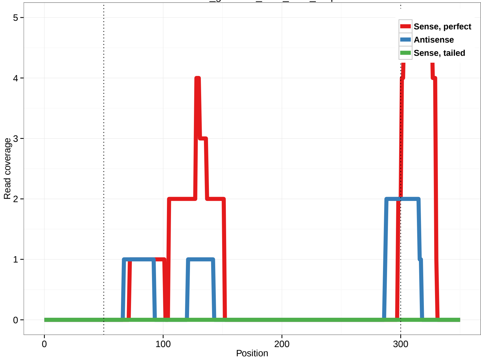
rheMac3_genscan_chr3_66.9_7.3p
