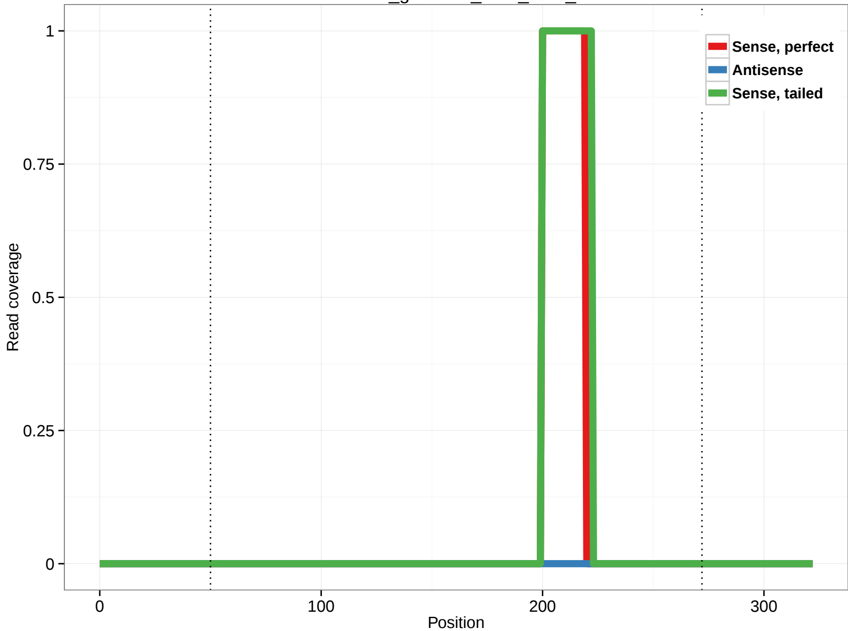
rheMac3_genscan_chr3_66.3_11
