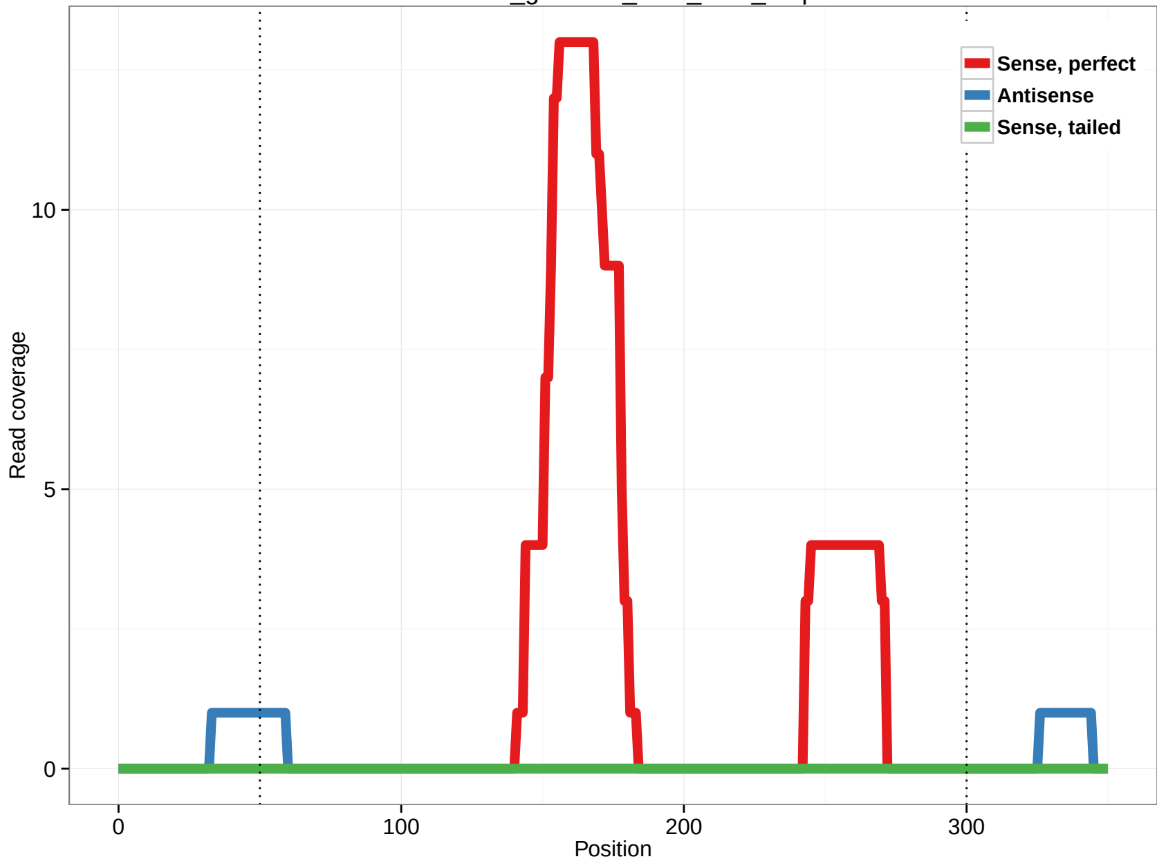
rheMac3_genscan_chr3_65.9_3.5p
