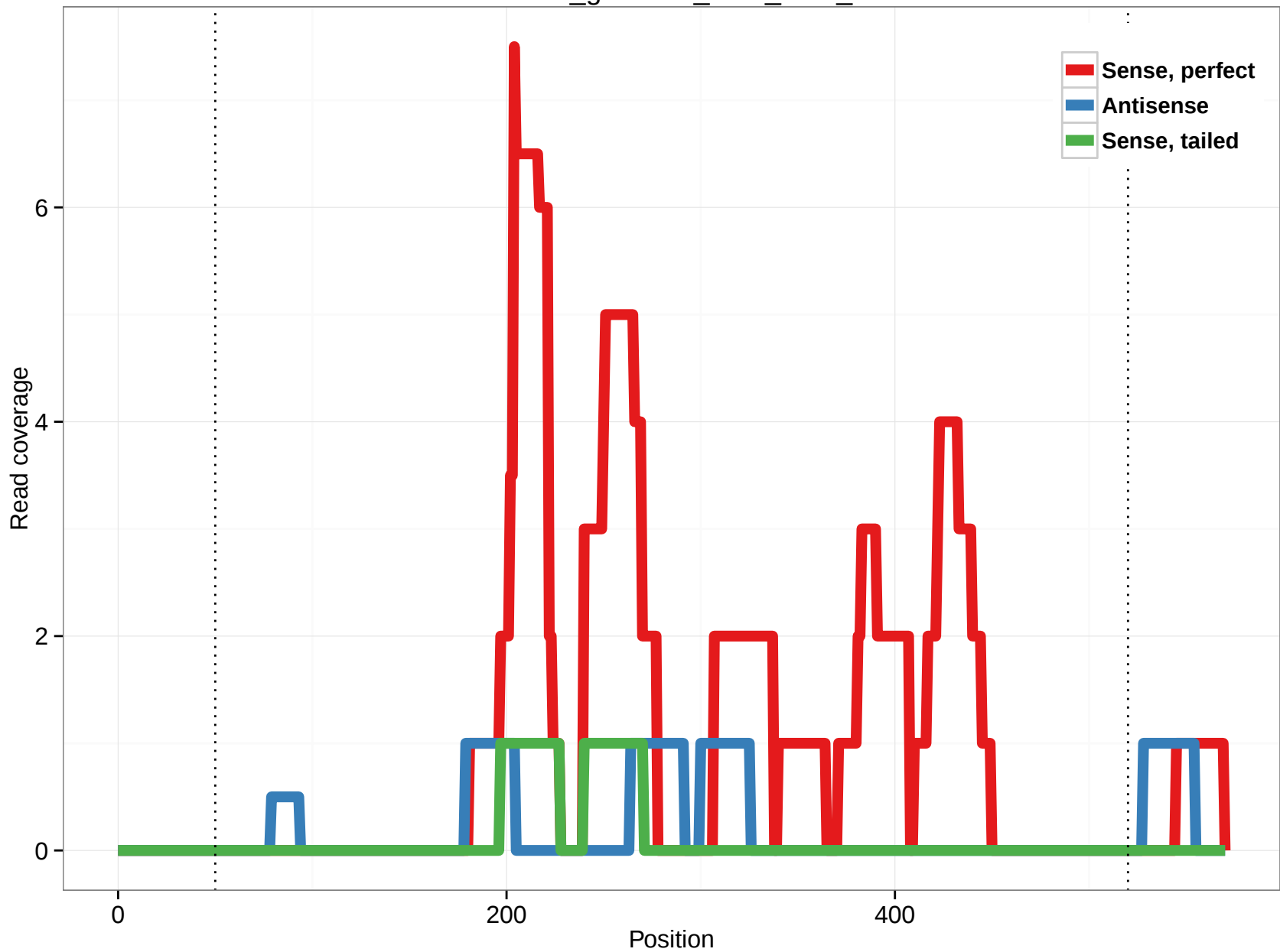
rheMac3_genscan_chr3_65.4_17
