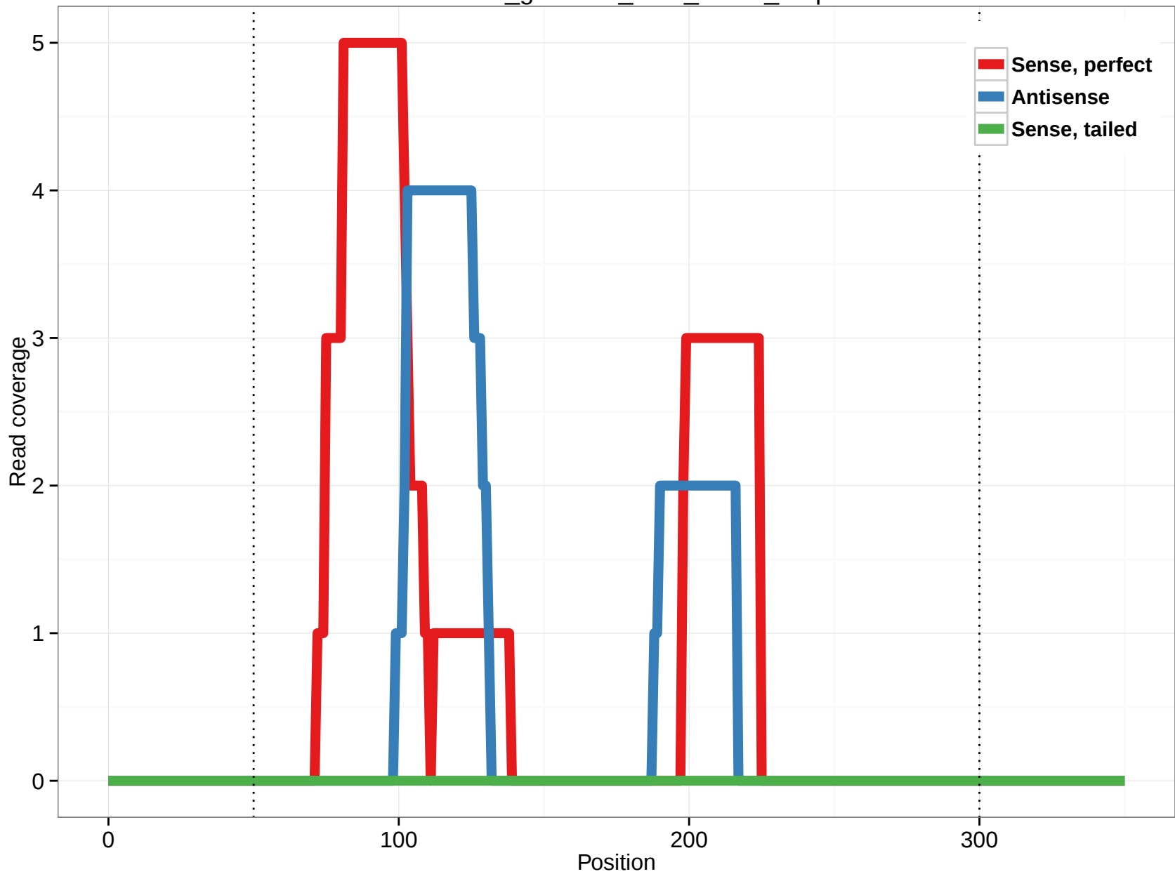
rheMac3_genscan_chr3_65.16_2.3p
