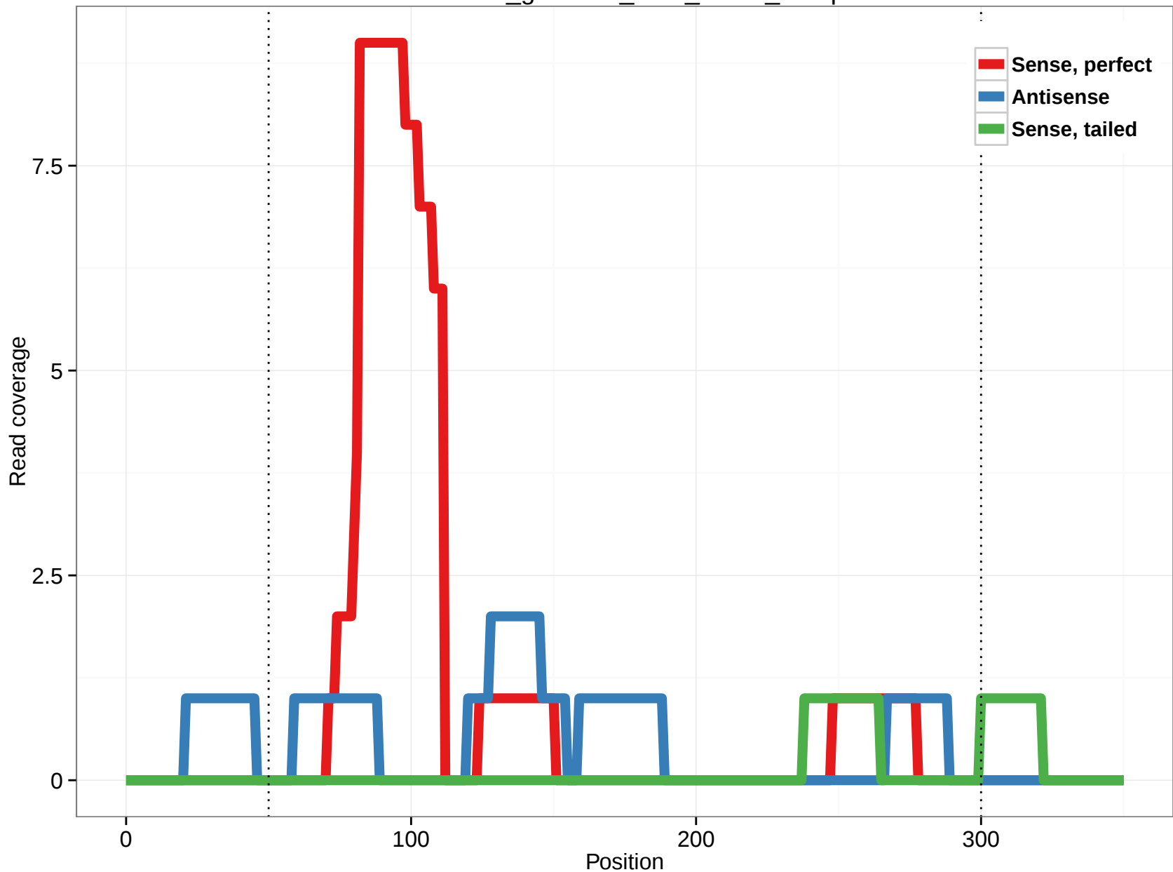
rheMac3_genscan_chr3_65.15_13.3p
