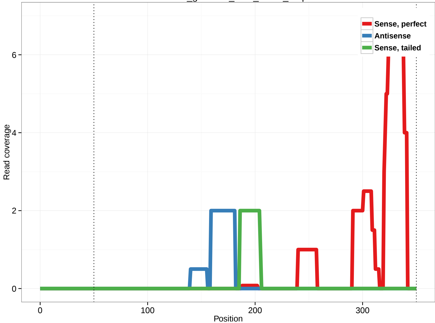
rheMac3_genscan_chr3_65.11_2.5p
