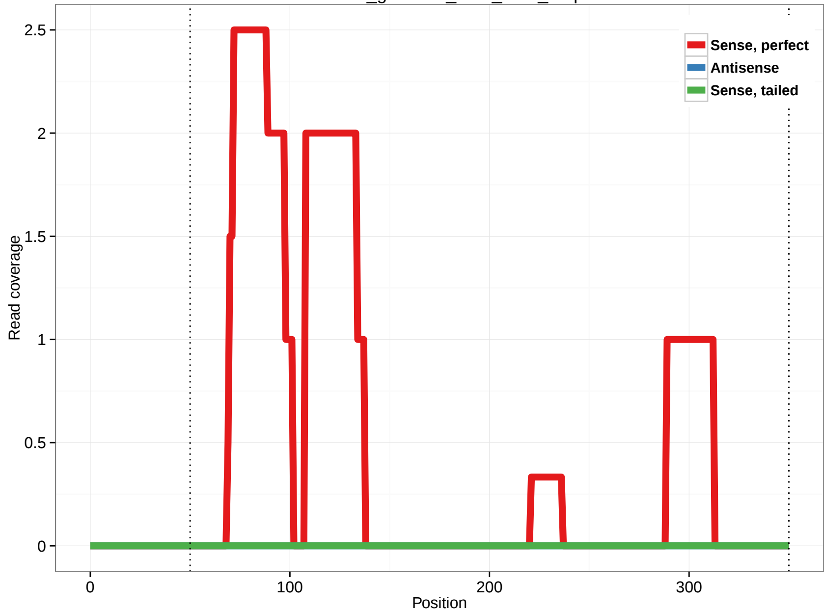
rheMac3_genscan_chr3_59.2_3.5p
