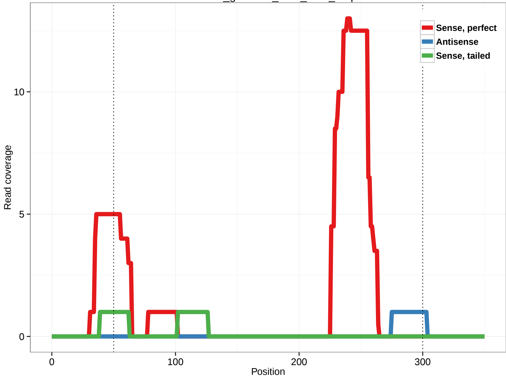
rheMac3_genscan_chr3_59.2_2.5p
