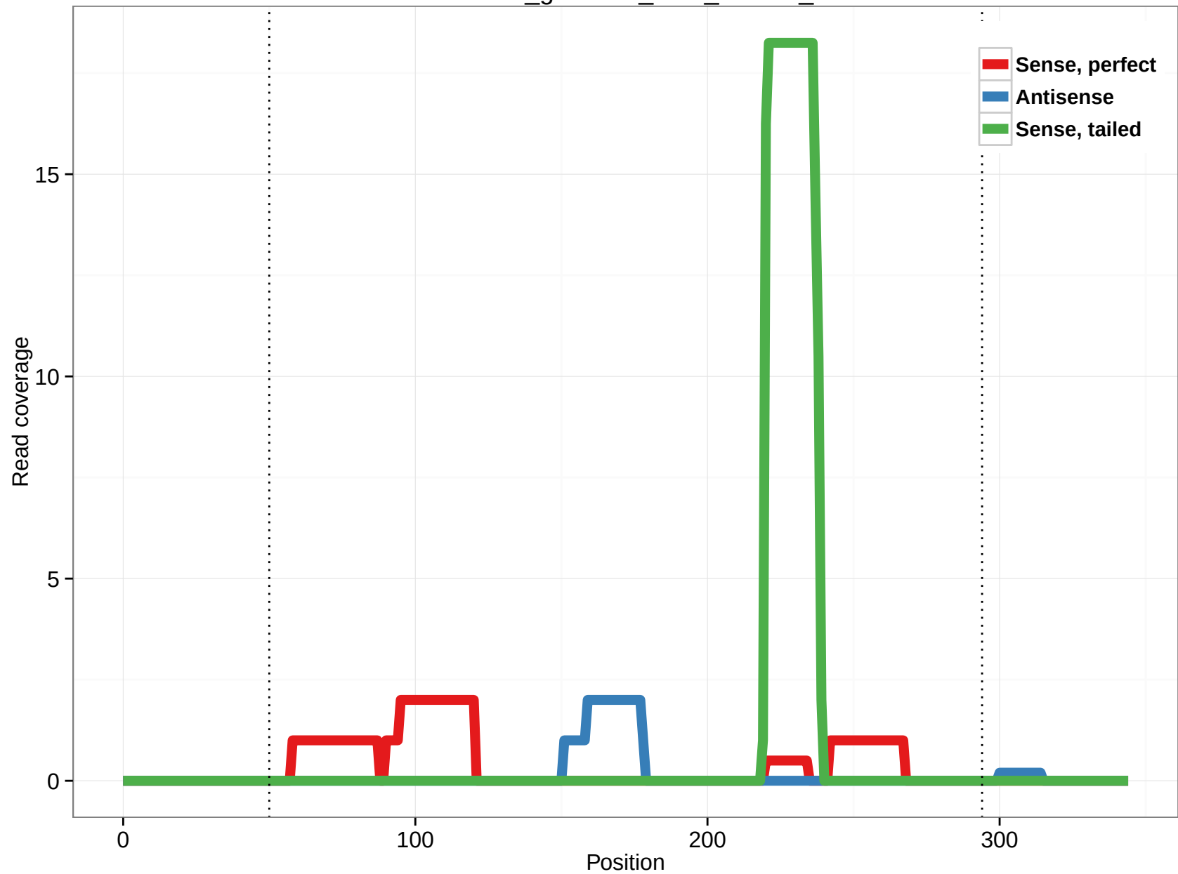
rheMac3_genscan_chr3_314.20_9
