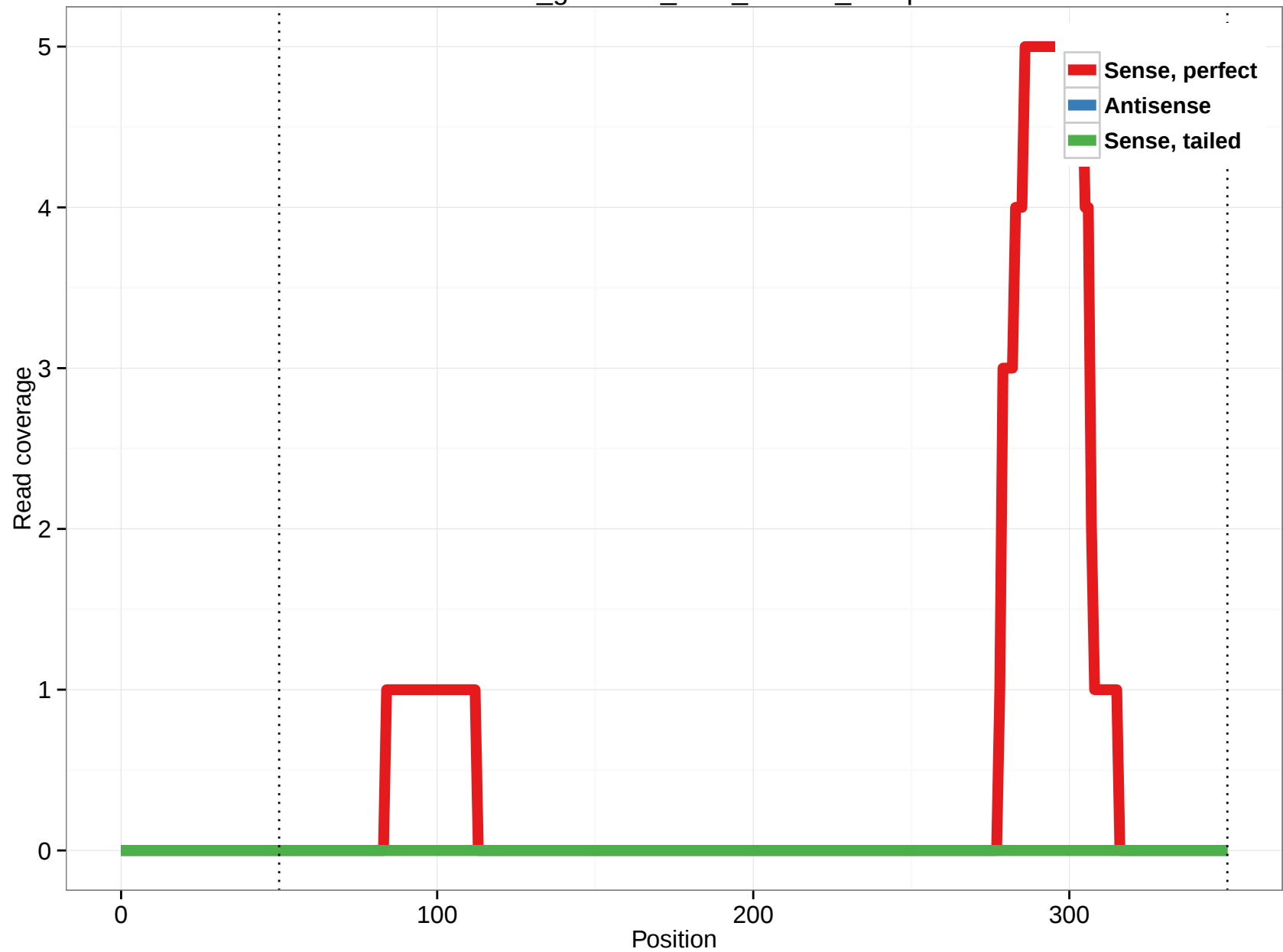
rheMac3_genscan_chr3_314.20_15.5p
