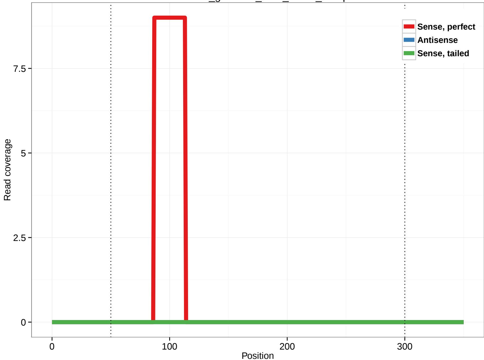
rheMac3_genscan_chr3_31.10_13.3p
